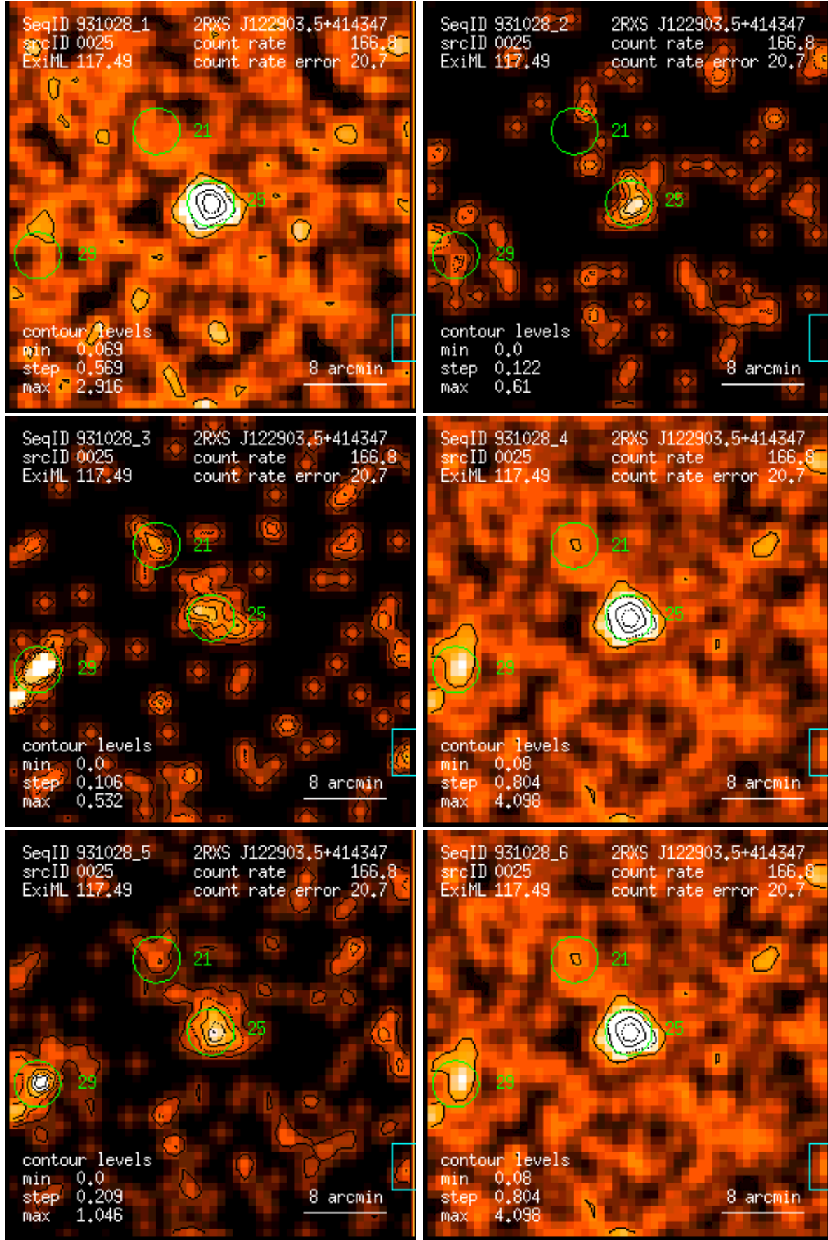
Figure 25: RASS 931028: detection 0025: band rate images, Gaussian filter: (1) PSPC channels 11 – 41, (2) 52 – 90, (3) 91 – 201, (4) 11 – 235, (5) 52 – 201, (6) 11 – 201. Broad band rates in counts/ks. Band rate contour levels in counts/ks/arcmin 2 .
