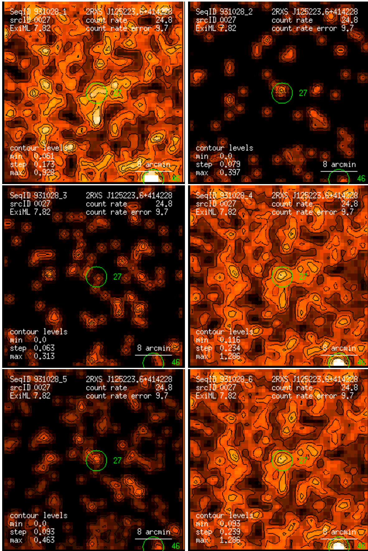
Figure 27: RASS 931028: detection 0027: band rate images, Gaussian filter: (1) PSPC channels 11 – 41, (2) 52 – 90, (3) 91 – 201, (4) 11 – 235, (5) 52 – 201, (6) 11 – 201. Broad band rates in counts/ks. Band rate contour levels in counts/ks/arcmin 2 .
