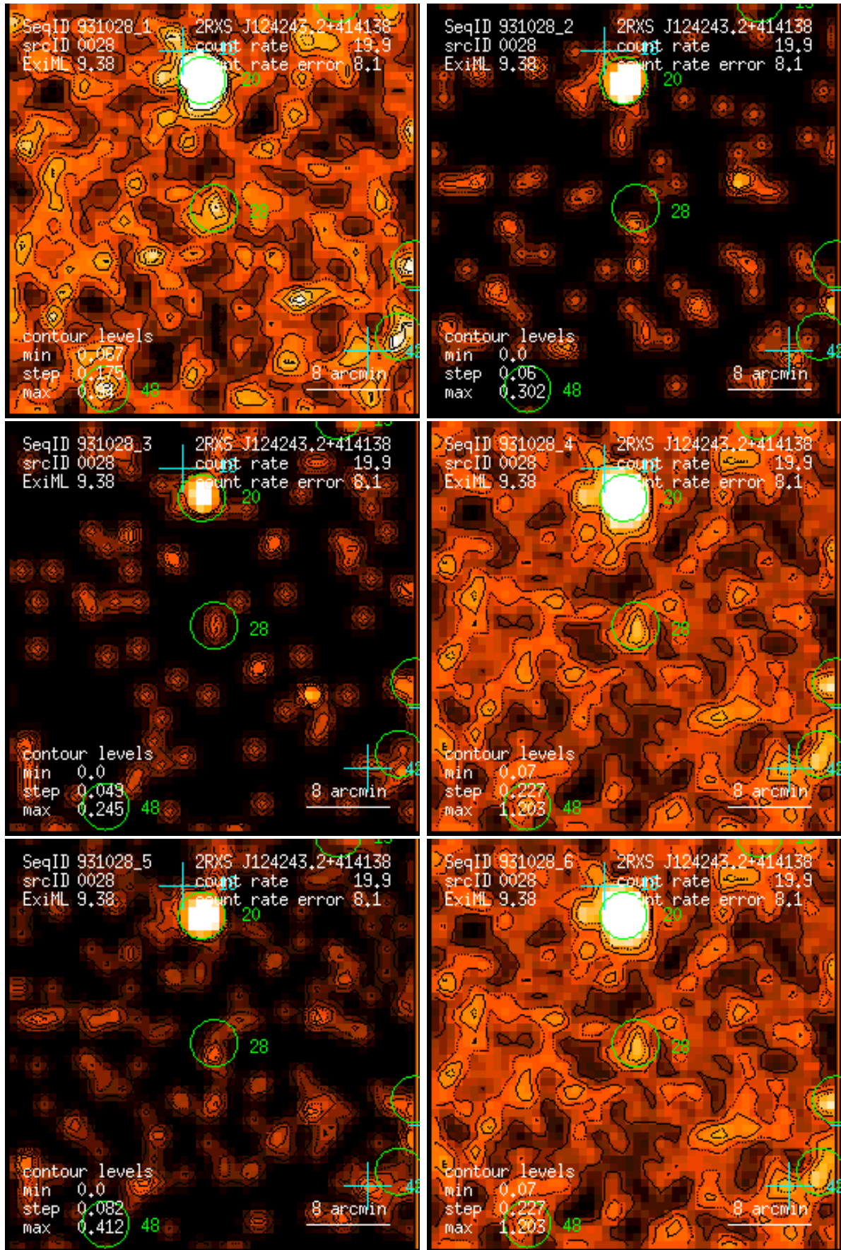
Figure 28: RASS 931028: detection 0028: band rate images, Gaussian filter: (1) PSPC channels 11 – 41, (2) 52 – 90, (3) 91 – 201, (4) 11 – 235, (5) 52 – 201, (6) 11 – 201. Broad band rates in counts/ks. Band rate contour levels in counts/ks/arcmin 2 .
