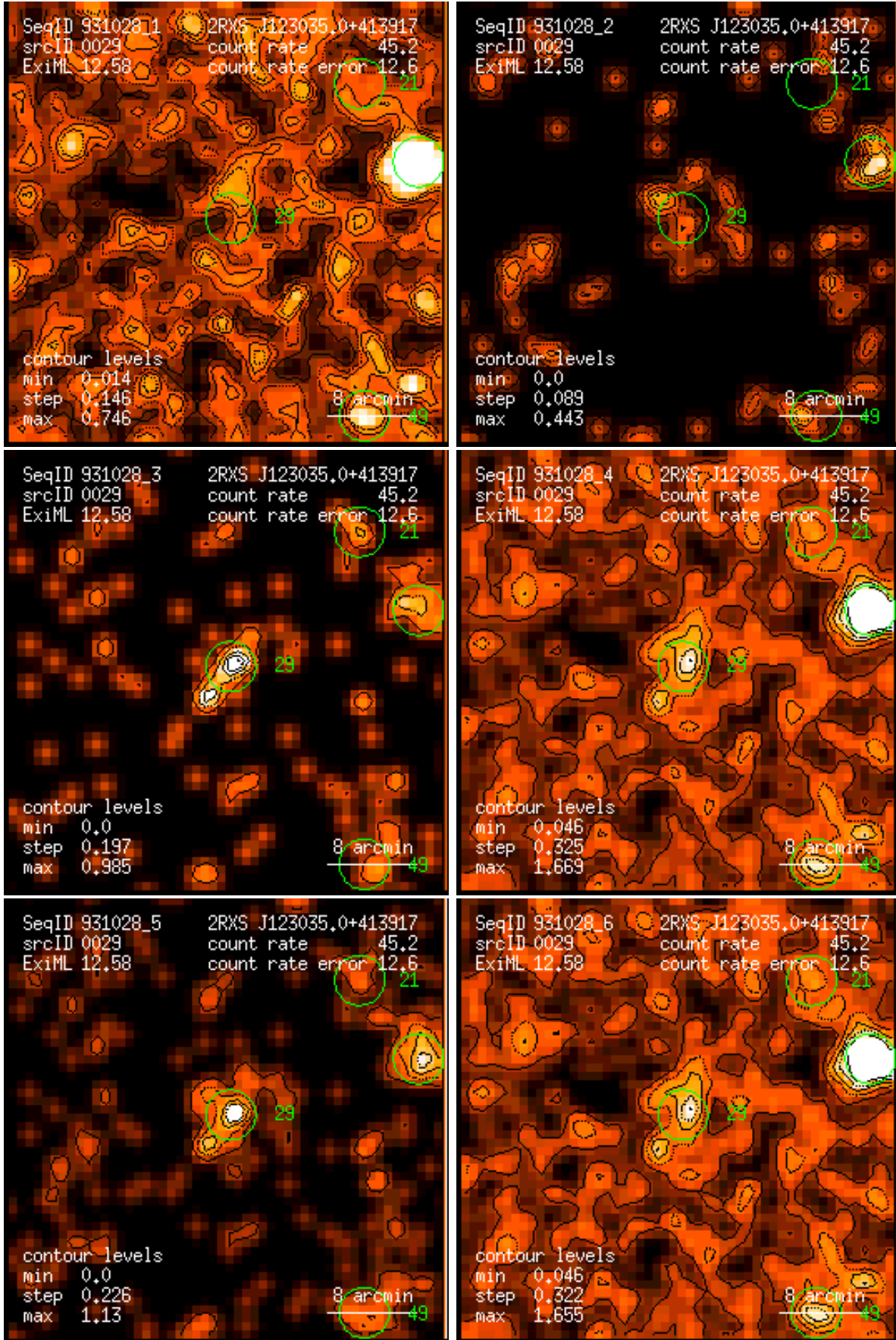
Figure 29: RASS 931028: detection 0029: band rate images, Gaussian filter: (1) PSPC channels 11 – 41, (2) 52 – 90, (3) 91 – 201, (4) 11 – 235, (5) 52 – 201, (6) 11 – 201. Broad band rates in counts/ks. Band rate contour levels in counts/ks/arcmin 2 .
