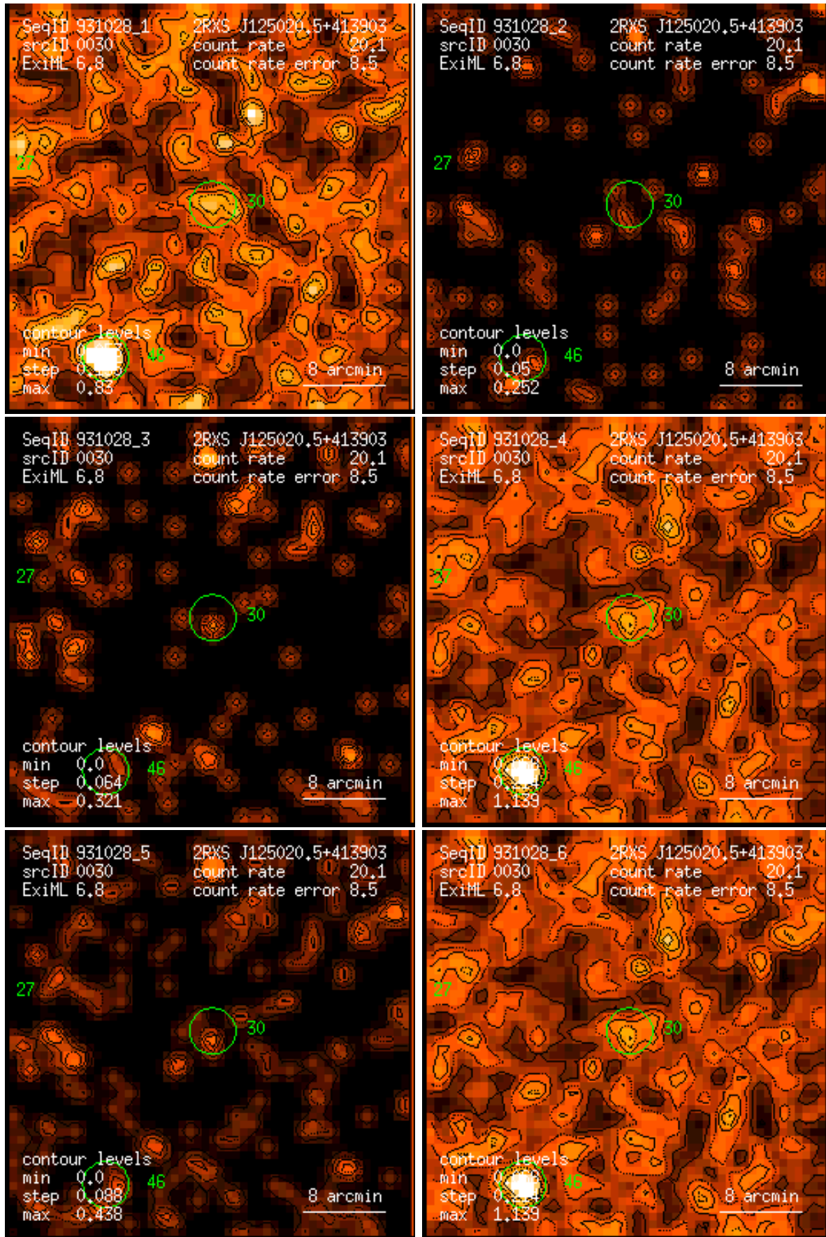
Figure 30: RASS 931028: detection 0030: band rate images, Gaussian filter: (1) PSPC channels 11 – 41, (2) 52 – 90, (3) 91 – 201, (4) 11 – 235, (5) 52 – 201, (6) 11 – 201. Broad band rates in counts/ks. Band rate contour levels in counts/ks/arcmin 2 .
