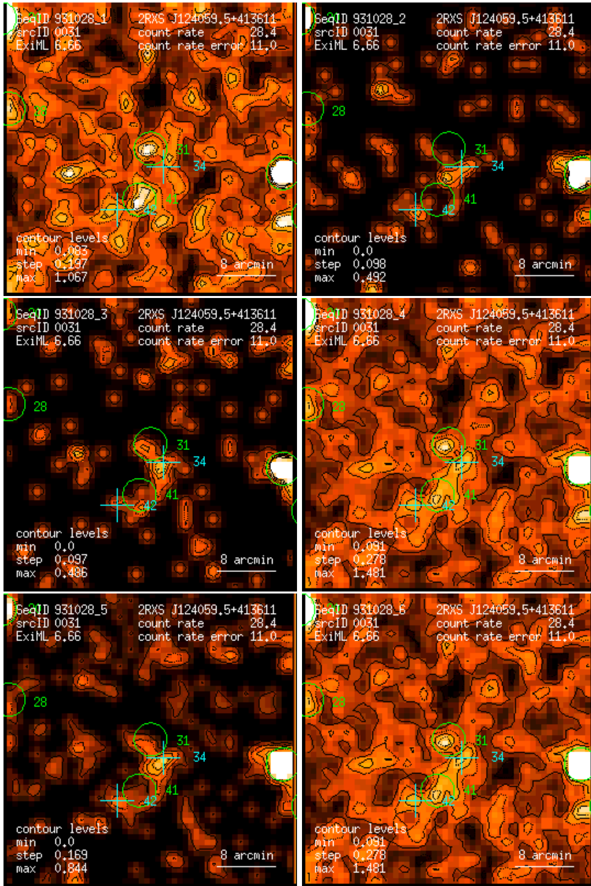
Figure 31: RASS 931028: detection 0031: band rate images, Gaussian filter: (1) PSPC channels 11 – 41, (2) 52 – 90, (3) 91 – 201, (4) 11 – 235, (5) 52 – 201, (6) 11 – 201. Broad band rates in counts/ks. Band rate contour levels in counts/ks/arcmin 2 .
