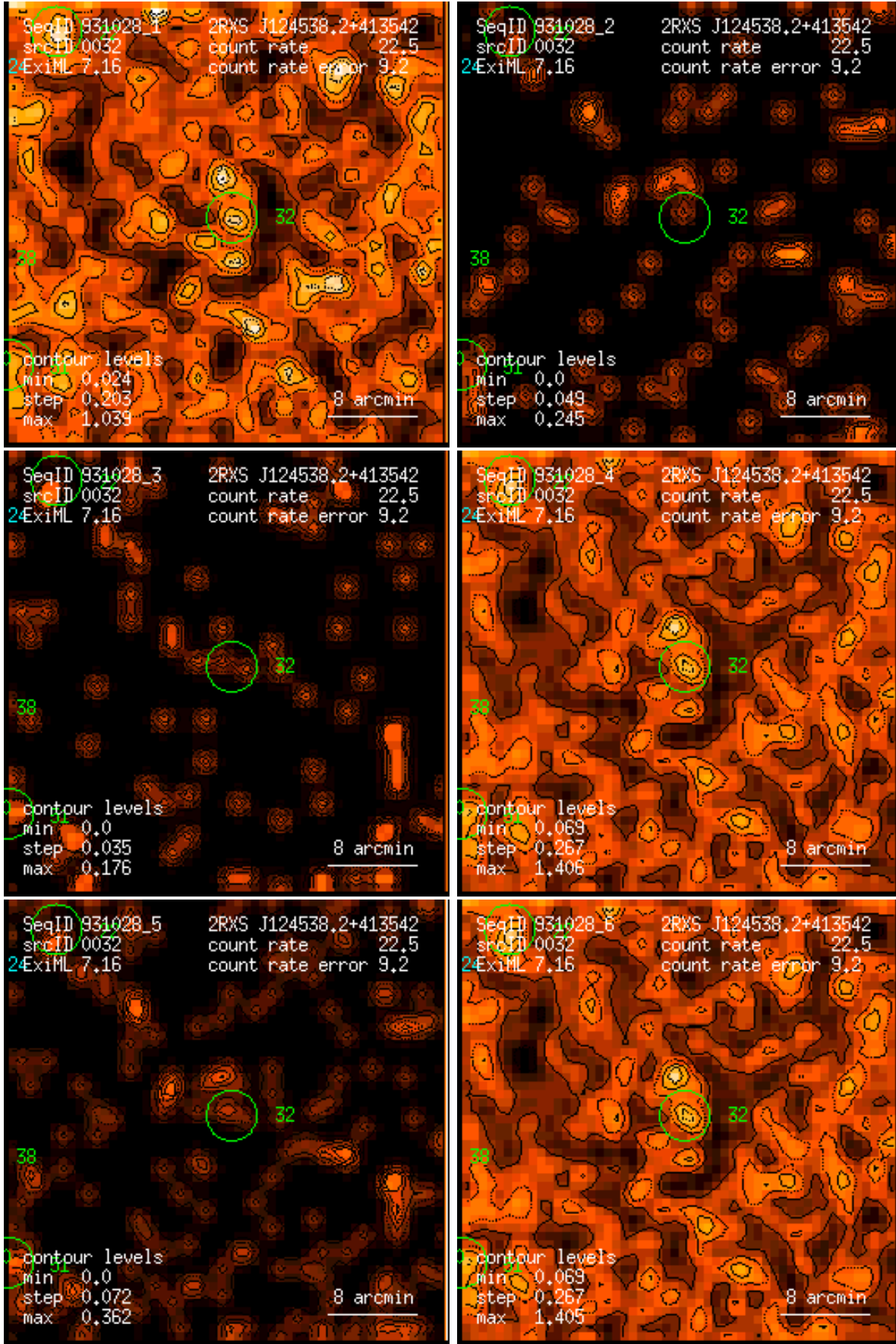
Figure 32: RASS 931028: detection 0032: band rate images, Gaussian filter: (1) PSPC channels 11 – 41, (2) 52 – 90, (3) 91 – 201, (4) 11 – 235, (5) 52 – 201, (6) 11 – 201. Broad band rates in counts/ks. Band rate contour levels in counts/ks/arcmin 2 .
