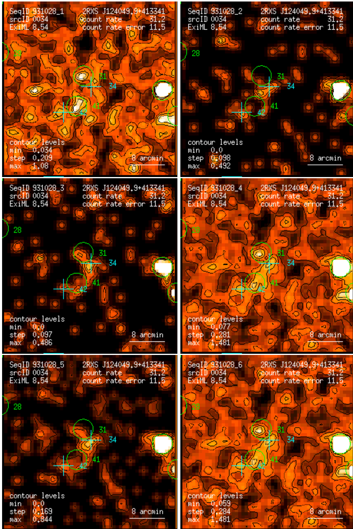
Figure 34: RASS 931028: detection 0034: band rate images, Gaussian filter: (1) PSPC channels 11 – 41, (2) 52 – 90, (3) 91 – 201, (4) 11 – 235, (5) 52 – 201, (6) 11 – 201. Broad band rates in counts/ks. Band rate contour levels in counts/ks/arcmin 2 .
