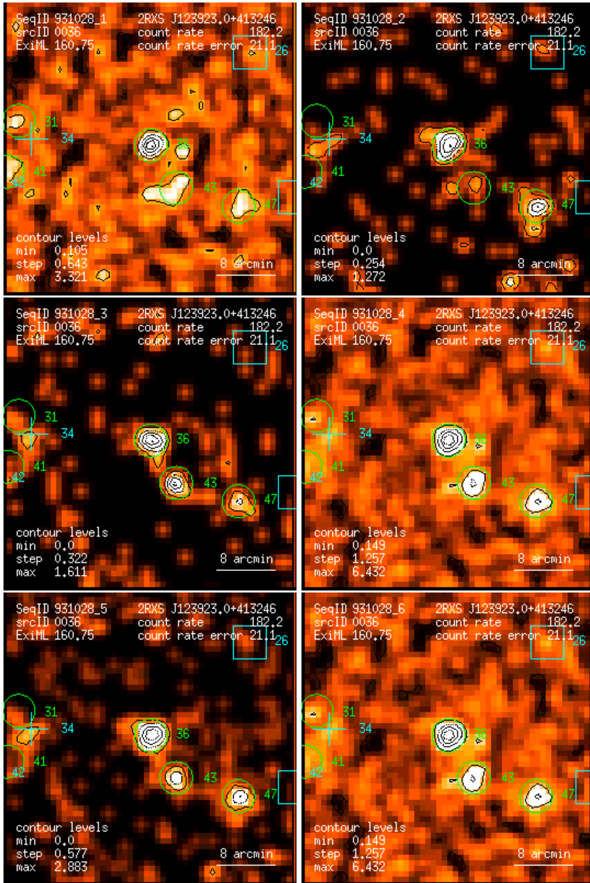
Figure 36: RASS 931028: detection 0036: band rate images, Gaussian filter: (1) PSPC channels 11 – 41, (2) 52 – 90, (3) 91 – 201, (4) 11 – 235, (5) 52 – 201, (6) 11 – 201. Broad band rates in counts/ks. Band rate contour levels in counts/ks/arcmin 2 .
