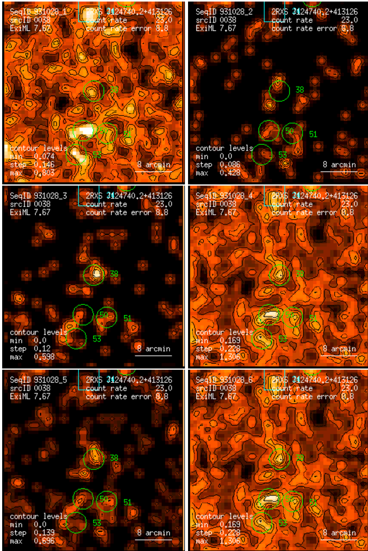
Figure 38: RASS 931028: detection 0038: band rate images, Gaussian filter: (1) PSPC channels 11 – 41, (2) 52 – 90, (3) 91 – 201, (4) 11 – 235, (5) 52 – 201, (6) 11 – 201. Broad band rates in counts/ks. Band rate contour levels in counts/ks/arcmin 2 .
