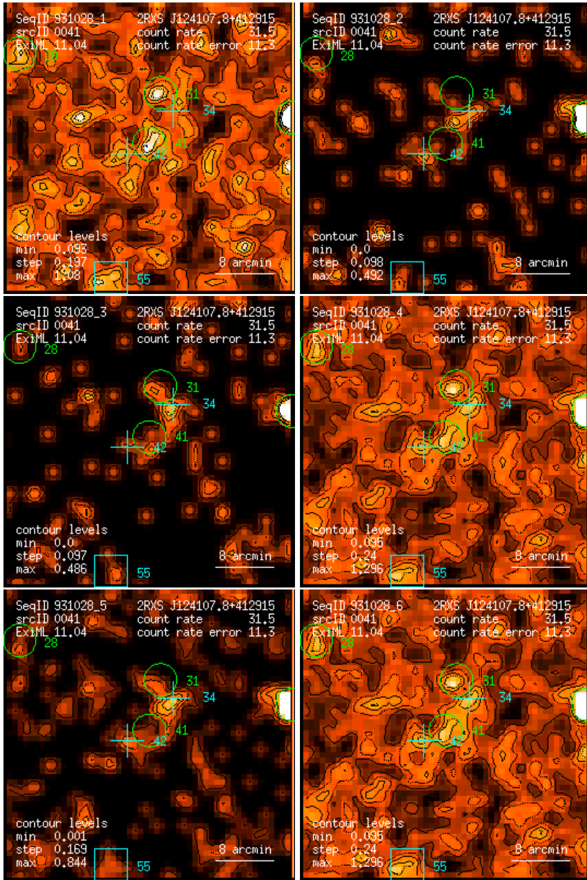
Figure 41: RASS 931028: detection 0041: band rate images, Gaussian filter: (1) PSPC channels 11 – 41, (2) 52 – 90, (3) 91 – 201, (4) 11 – 235, (5) 52 – 201, (6) 11 – 201. Broad band rates in counts/ks. Band rate contour levels in counts/ks/arcmin 2 .
