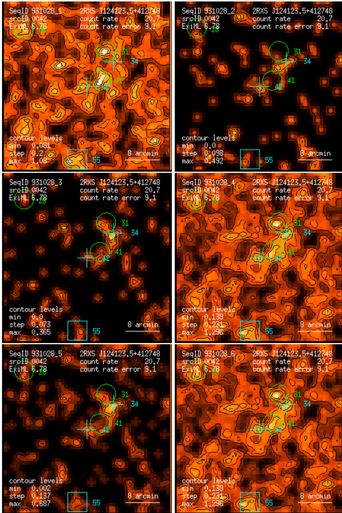
Figure 42: RASS 931028: detection 0042: band rate images, Gaussian filter: (1) PSPC channels 11 – 41, (2) 52 – 90, (3) 91 – 201, (4) 11 – 235, (5) 52 – 201, (6) 11 – 201. Broad band rates in counts/ks. Band rate contour levels in counts/ks/arcmin 2 .
