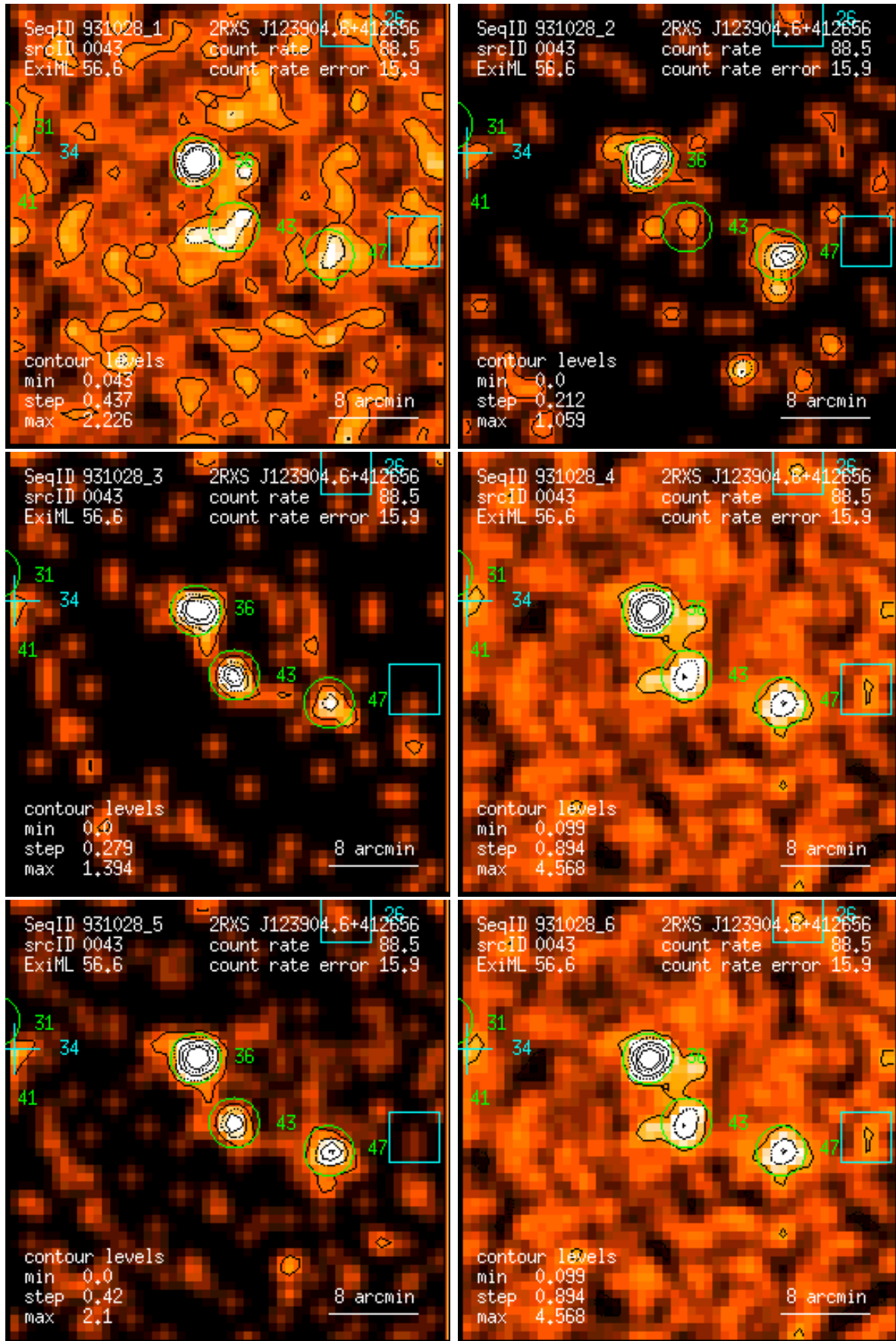
Figure 43: RASS 931028: detection 0043: band rate images, Gaussian filter: (1) PSPC channels 11 – 41, (2) 52 – 90, (3) 91 – 201, (4) 11 – 235, (5) 52 – 201, (6) 11 – 201. Broad band rates in counts/ks. Band rate contour levels in counts/ks/arcmin 2 .
