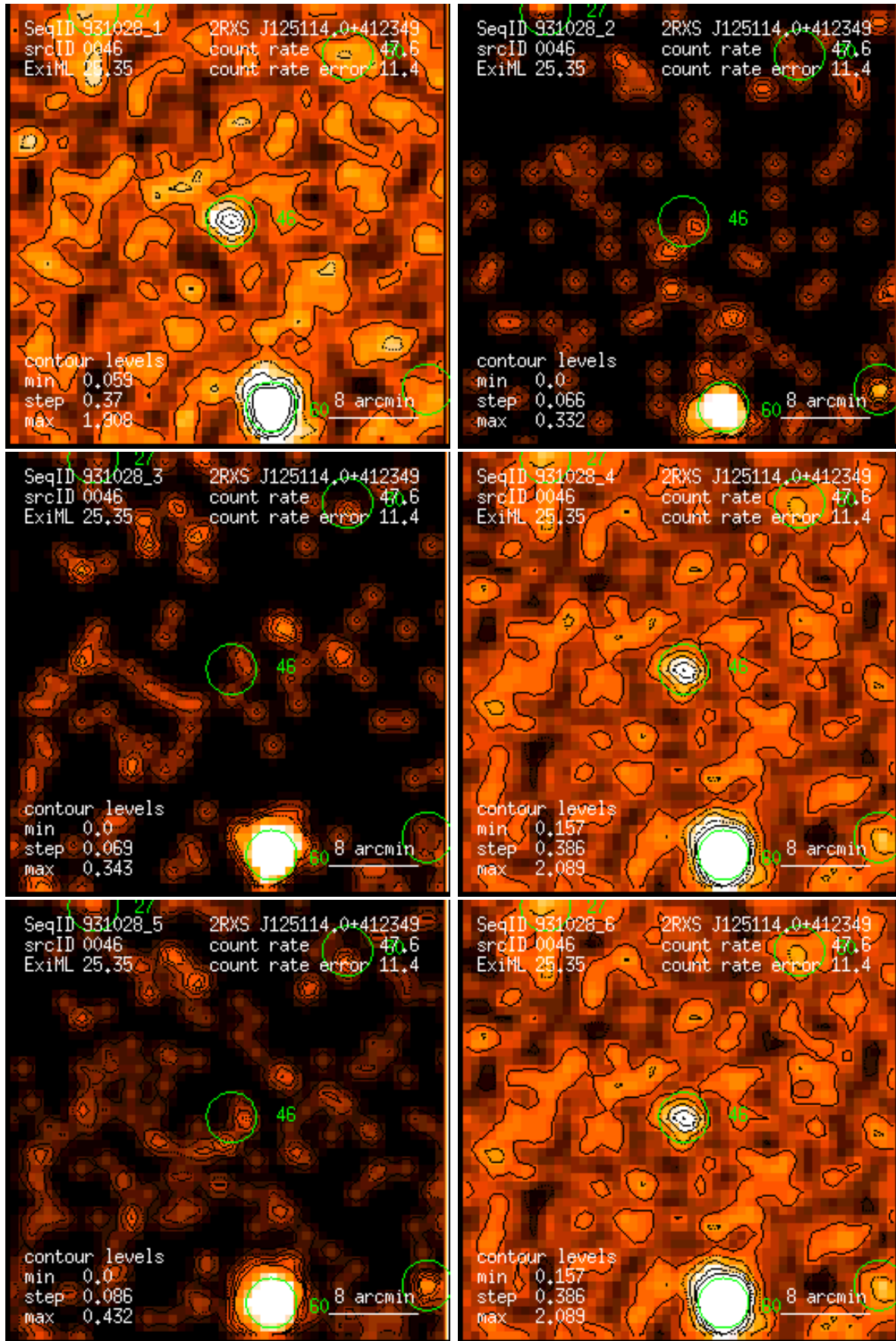
Figure 46: RASS 931028: detection 0046: band rate images, Gaussian filter: (1) PSPC channels 11 – 41, (2) 52 – 90, (3) 91 – 201, (4) 11 – 235, (5) 52 – 201, (6) 11 – 201. Broad band rates in counts/ks. Band rate contour levels in counts/ks/arcmin 2 .
