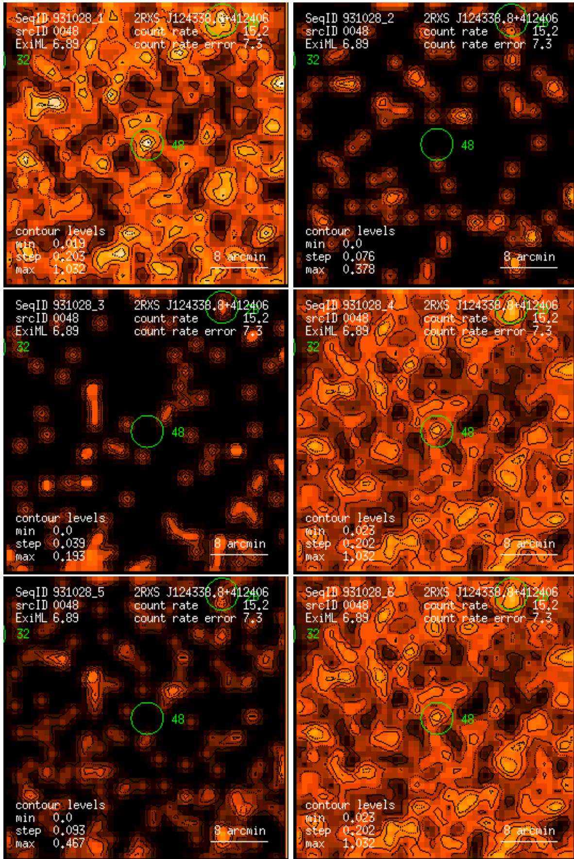
Figure 48: RASS 931028: detection 0048: band rate images, Gaussian filter: (1) PSPC channels 11 – 41, (2) 52 – 90, (3) 91 – 201, (4) 11 – 235, (5) 52 – 201, (6) 11 – 201. Broad band rates in counts/ks. Band rate contour levels in counts/ks/arcmin 2 .
