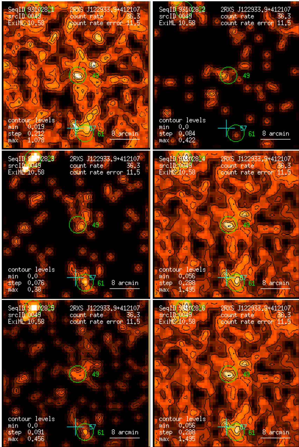
Figure 49: RASS 931028: detection 0049: band rate images, Gaussian filter: (1) PSPC channels 11 – 41, (2) 52 – 90, (3) 91 – 201, (4) 11 – 235, (5) 52 – 201, (6) 11 – 201. Broad band rates in counts/ks. Band rate contour levels in counts/ks/arcmin 2 .
