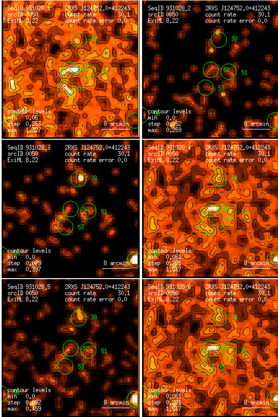
Figure 50: RASS 931028: detection 0050: band rate images, Gaussian filter: (1) PSPC channels 11 – 41, (2) 52 – 90, (3) 91 – 201, (4) 11 – 235, (5) 52 – 201, (6) 11 – 201. Broad band rates in counts/ks. Band rate contour levels in counts/ks/arcmin 2 .
