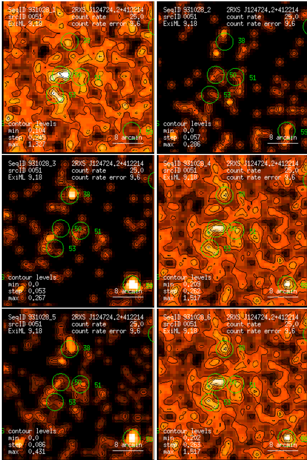
Figure 51: RASS 931028: detection 0051: band rate images, Gaussian filter: (1) PSPC channels 11 – 41, (2) 52 – 90, (3) 91 – 201, (4) 11 – 235, (5) 52 – 201, (6) 11 – 201. Broad band rates in counts/ks. Band rate contour levels in counts/ks/arcmin 2 .
