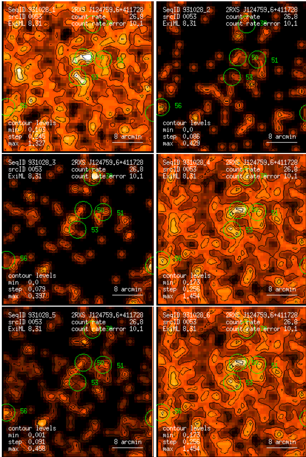
Figure 53: RASS 931028: detection 0053: band rate images, Gaussian filter: (1) PSPC channels 11 – 41, (2) 52 – 90, (3) 91 – 201, (4) 11 – 235, (5) 52 – 201, (6) 11 – 201. Broad band rates in counts/ks. Band rate contour levels in counts/ks/arcmin 2 .
