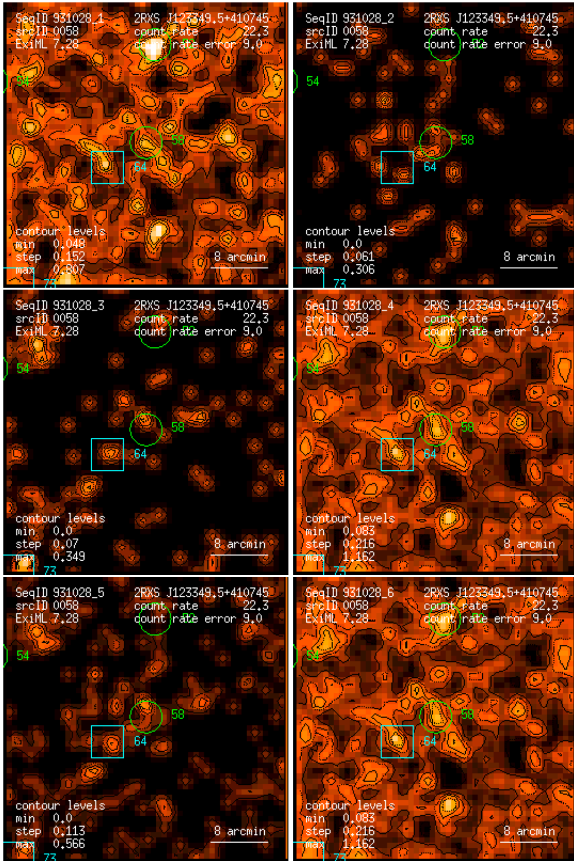
Figure 58: RASS 931028: detection 0058: band rate images, Gaussian filter: (1) PSPC channels 11 – 41, (2) 52 – 90, (3) 91 – 201, (4) 11 – 235, (5) 52 – 201, (6) 11 – 201. Broad band rates in counts/ks. Band rate contour levels in counts/ks/arcmin 2 .
