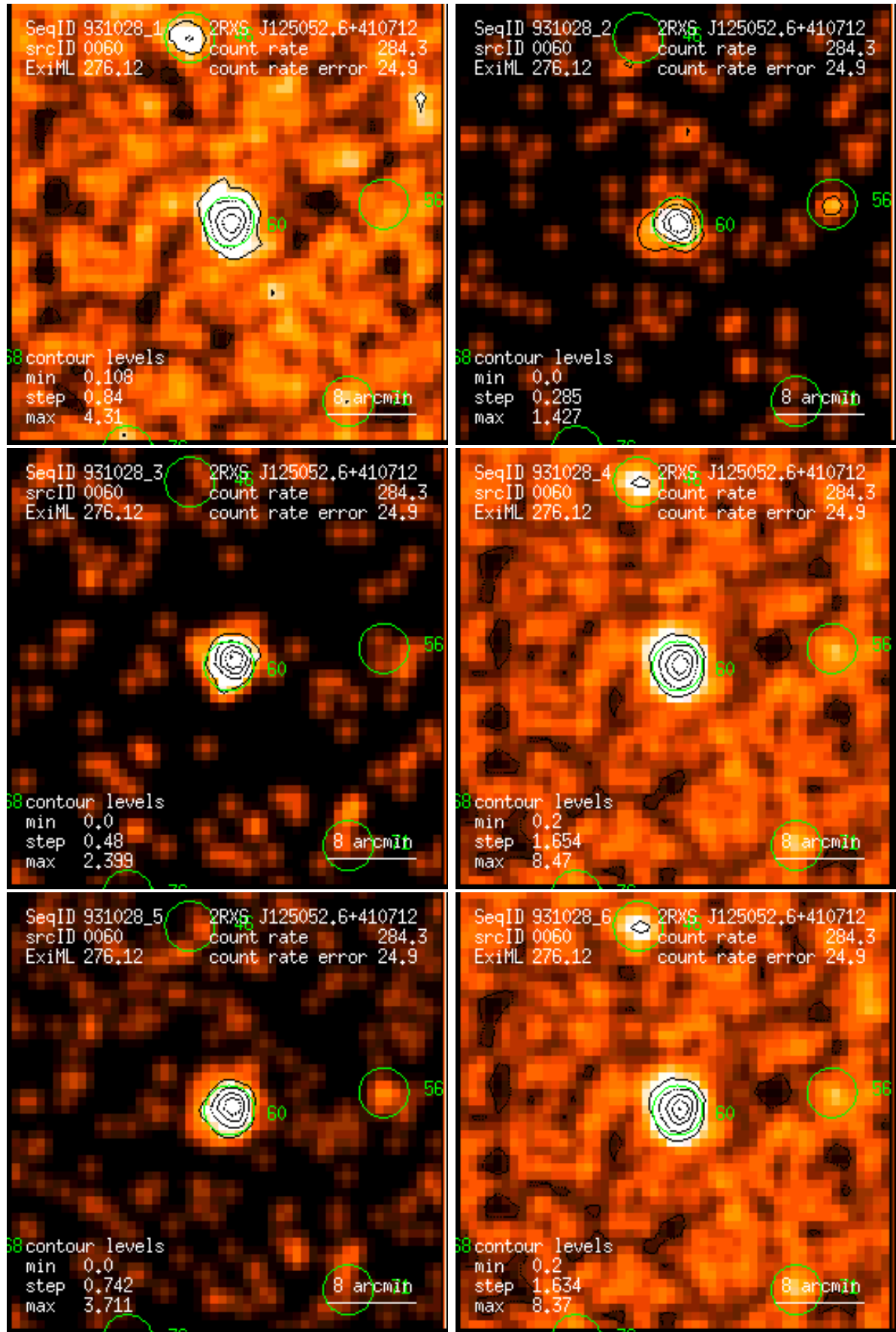
Figure 60: RASS 931028: detection 0060: band rate images, Gaussian filter: (1) PSPC channels 11 – 41, (2) 52 – 90, (3) 91 – 201, (4) 11 – 235, (5) 52 – 201, (6) 11 – 201. Broad band rates in counts/ks. Band rate contour levels in counts/ks/arcmin 2 .
