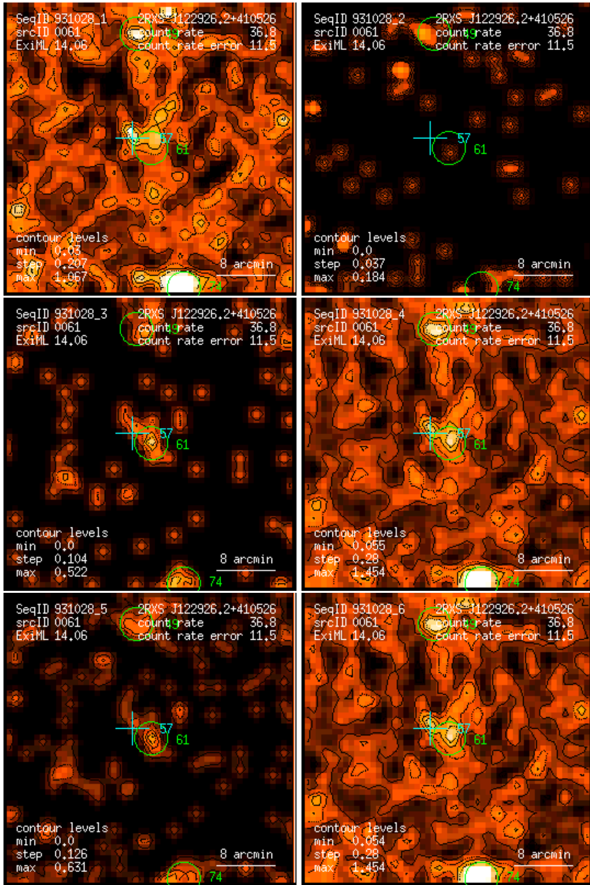
Figure 61: RASS 931028: detection 0061: band rate images, Gaussian filter: (1) PSPC channels 11 – 41, (2) 52 – 90, (3) 91 – 201, (4) 11 – 235, (5) 52 – 201, (6) 11 – 201. Broad band rates in counts/ks. Band rate contour levels in counts/ks/arcmin 2 .
