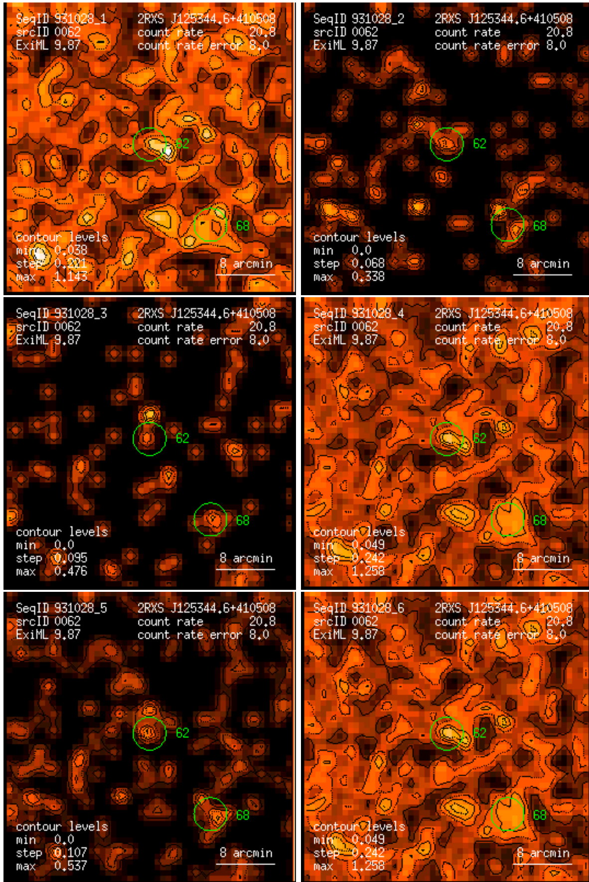
Figure 62: RASS 931028: detection 0062: band rate images, Gaussian filter: (1) PSPC channels 11 – 41, (2) 52 – 90, (3) 91 – 201, (4) 11 – 235, (5) 52 – 201, (6) 11 – 201. Broad band rates in counts/ks. Band rate contour levels in counts/ks/arcmin 2 .
