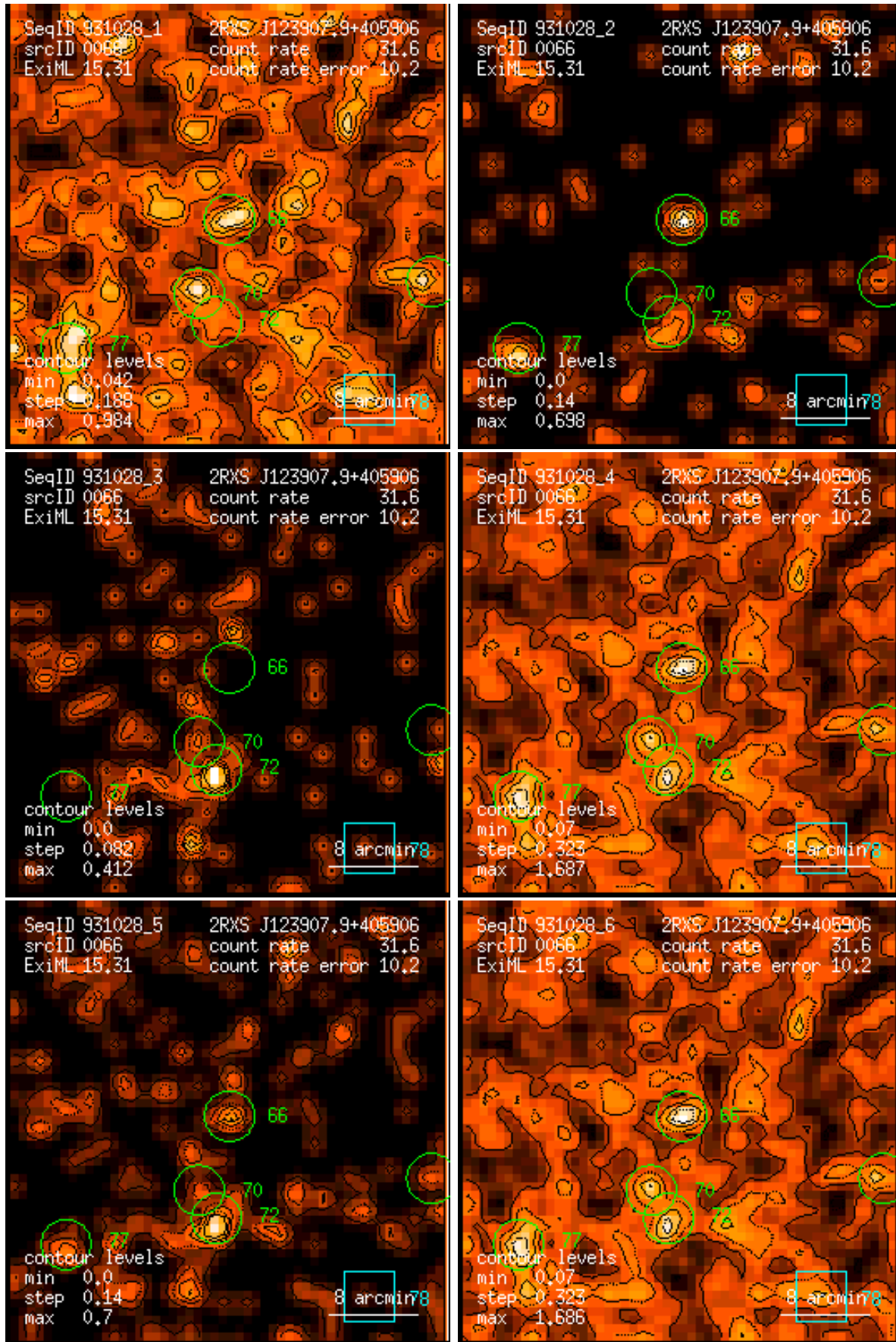
Figure 66: RASS 931028: detection 0066: band rate images, Gaussian filter: (1) PSPC channels 11 – 41, (2) 52 – 90, (3) 91 – 201, (4) 11 – 235, (5) 52 – 201, (6) 11 – 201. Broad band rates in counts/ks. Band rate contour levels in counts/ks/arcmin 2 .
