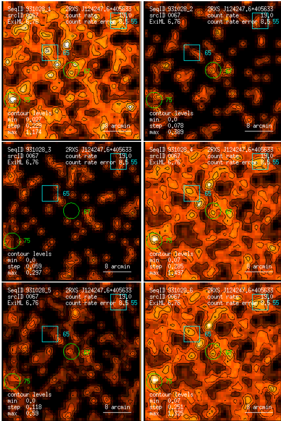
Figure 67: RASS 931028: detection 0067: band rate images, Gaussian filter: (1) PSPC channels 11 – 41, (2) 52 – 90, (3) 91 – 201, (4) 11 – 235, (5) 52 – 201, (6) 11 – 201. Broad band rates in counts/ks. Band rate contour levels in counts/ks/arcmin 2 .
