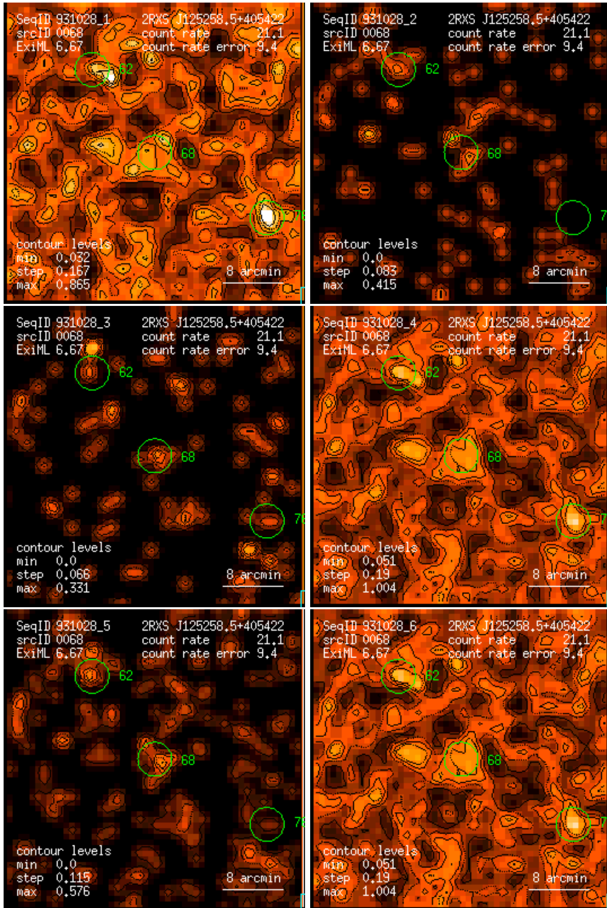
Figure 68: RASS 931028: detection 0068: band rate images, Gaussian filter: (1) PSPC channels 11 – 41, (2) 52 – 90, (3) 91 – 201, (4) 11 – 235, (5) 52 – 201, (6) 11 – 201. Broad band rates in counts/ks. Band rate contour levels in counts/ks/arcmin 2 .
