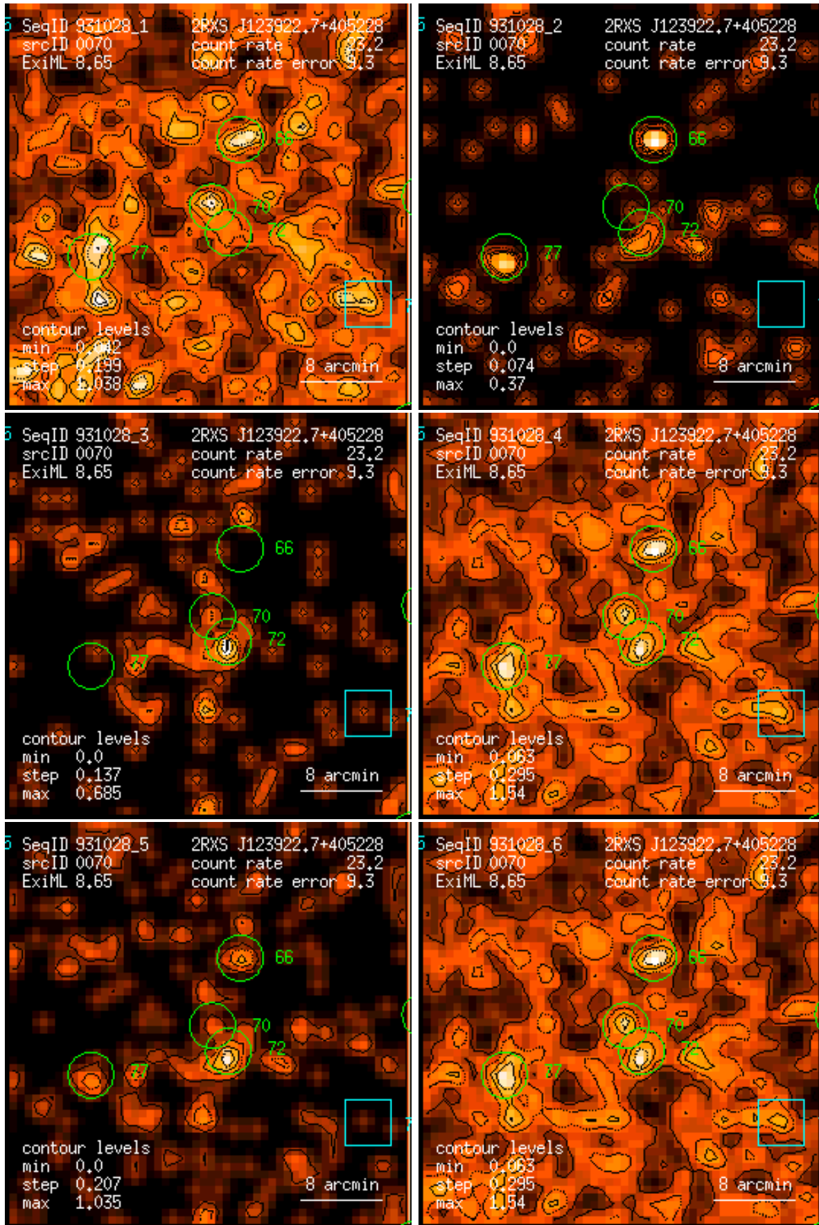
Figure 70: RASS 931028: detection 0070: band rate images, Gaussian filter: (1) PSPC channels 11 – 41, (2) 52 – 90, (3) 91 – 201, (4) 11 – 235, (5) 52 – 201, (6) 11 – 201. Broad band rates in counts/ks. Band rate contour levels in counts/ks/arcmin 2 .
