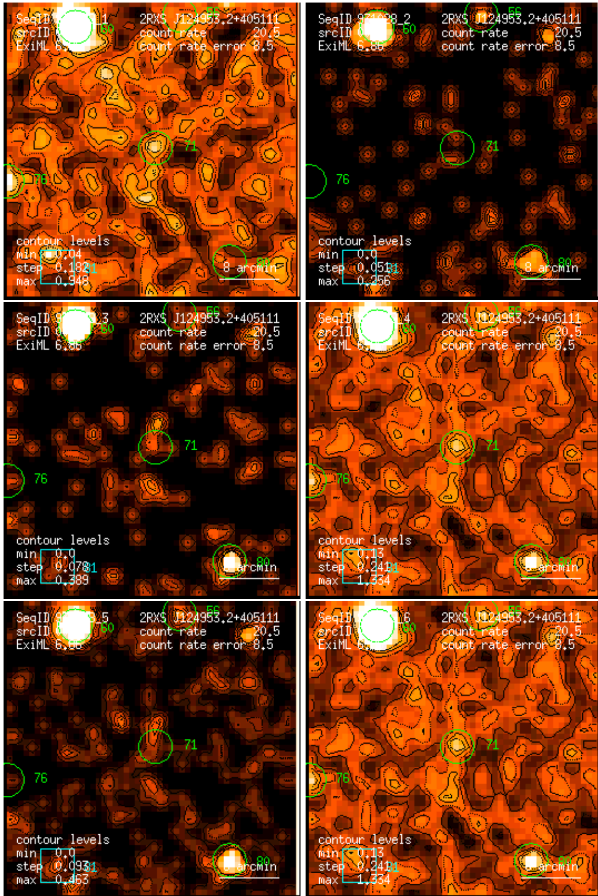
Figure 71: RASS 931028: detection 0071: band rate images, Gaussian filter: (1) PSPC channels 11 – 41, (2) 52 – 90, (3) 91 – 201, (4) 11 – 235, (5) 52 – 201, (6) 11 – 201. Broad band rates in counts/ks. Band rate contour levels in counts/ks/arcmin 2 .
