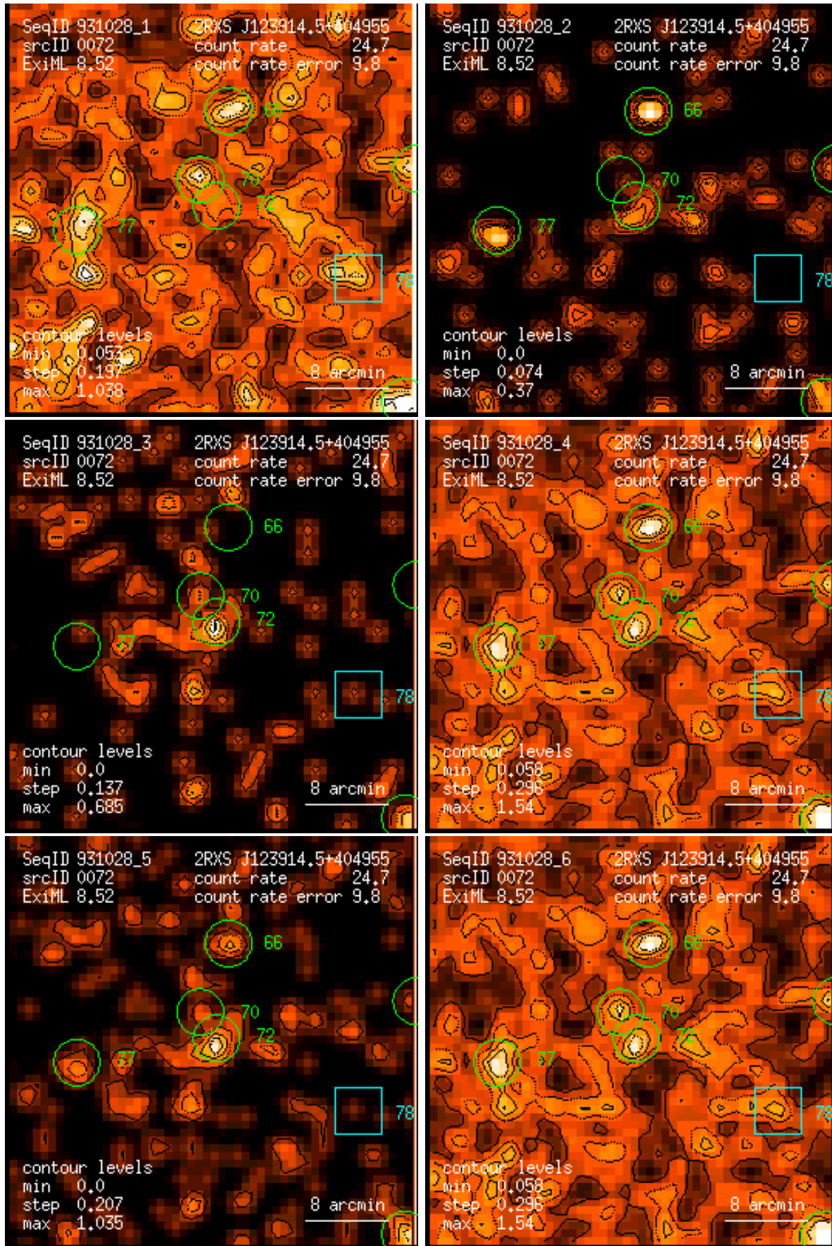
Figure 72: RASS 931028: detection 0072: band rate images, Gaussian filter: (1) PSPC channels 11 – 41, (2) 52 – 90, (3) 91 – 201, (4) 11 – 235, (5) 52 – 201, (6) 11 – 201. Broad band rates in counts/ks. Band rate contour levels in counts/ks/arcmin 2 .
