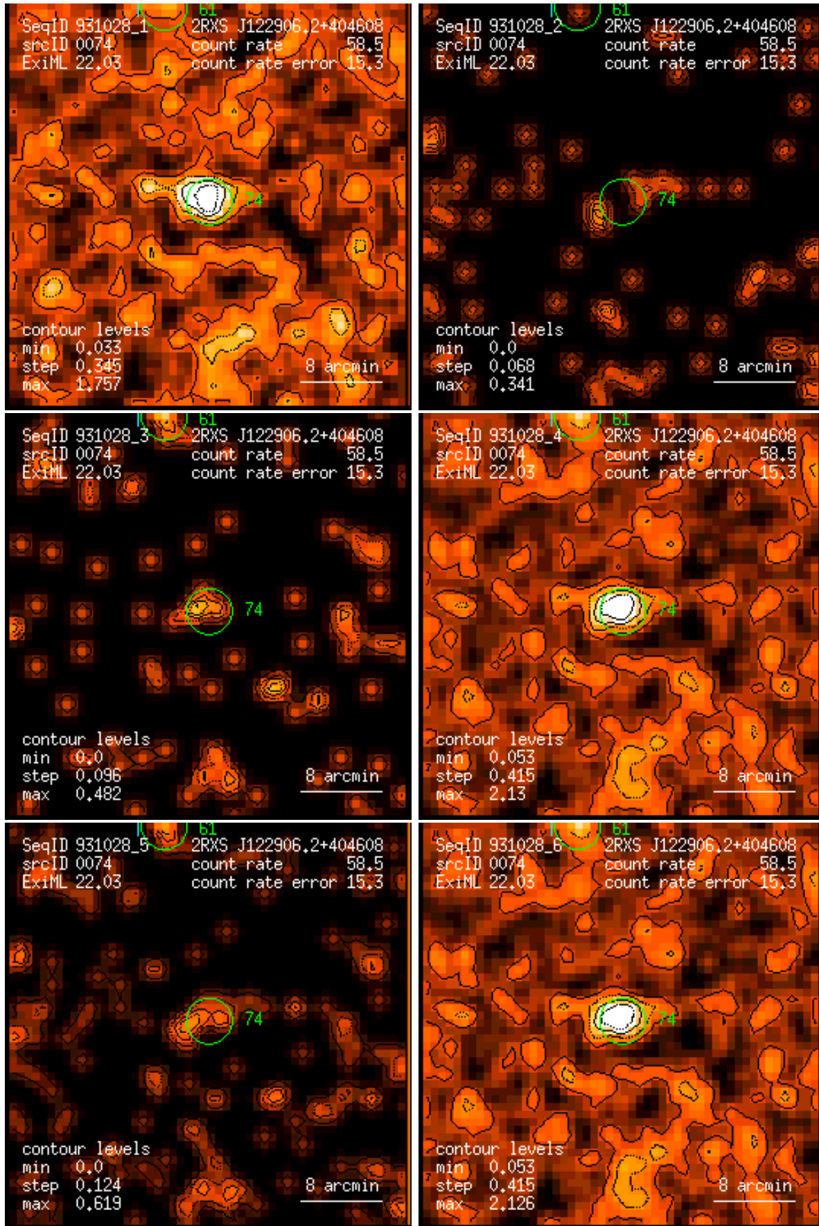
Figure 74: RASS 931028: detection 0074: band rate images, Gaussian filter: (1) PSPC channels 11 – 41, (2) 52 – 90, (3) 91 – 201, (4) 11 – 235, (5) 52 – 201, (6) 11 – 201. Broad band rates in counts/ks. Band rate contour levels in counts/ks/arcmin 2 .
