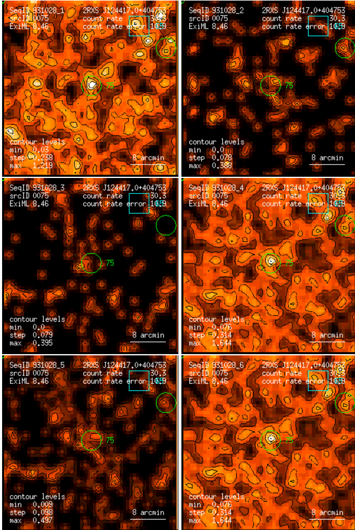
Figure 75: RASS 931028: detection 0075: band rate images, Gaussian filter: (1) PSPC channels 11 – 41, (2) 52 – 90, (3) 91 – 201, (4) 11 – 235, (5) 52 – 201, (6) 11 – 201. Broad band rates in counts/ks. Band rate contour levels in counts/ks/arcmin 2 .
