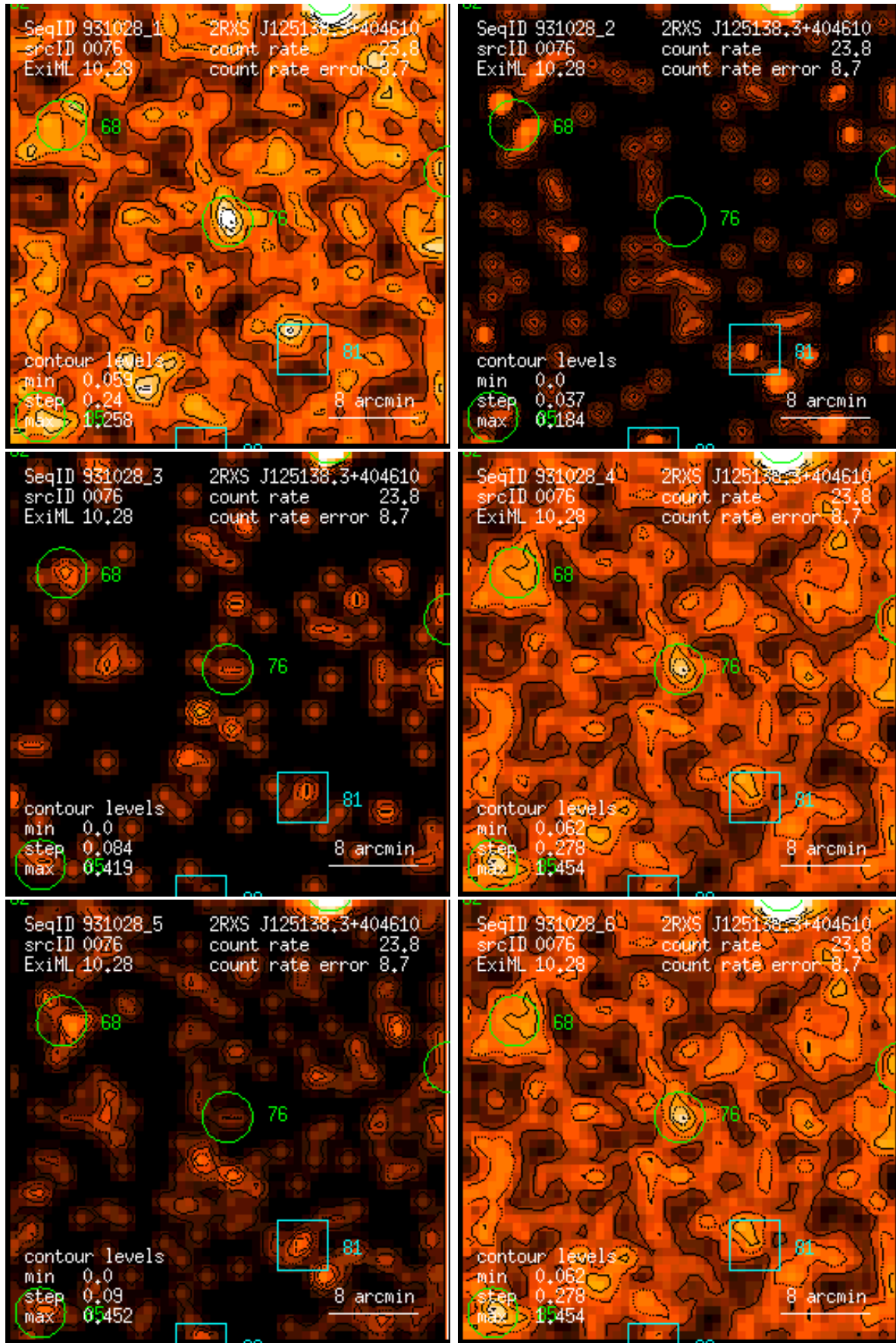
Figure 76: RASS 931028: detection 0076: band rate images, Gaussian filter: (1) PSPC channels 11 – 41, (2) 52 – 90, (3) 91 – 201, (4) 11 – 235, (5) 52 – 201, (6) 11 – 201. Broad band rates in counts/ks. Band rate contour levels in counts/ks/arcmin 2 .
