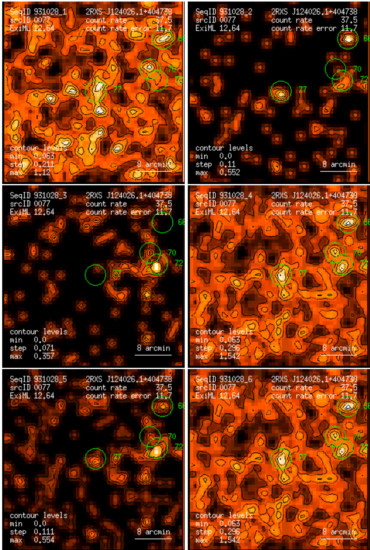
Figure 77: RASS 931028: detection 0077: band rate images, Gaussian filter: (1) PSPC channels 11 – 41, (2) 52 – 90, (3) 91 – 201, (4) 11 – 235, (5) 52 – 201, (6) 11 – 201. Broad band rates in counts/ks. Band rate contour levels in counts/ks/arcmin 2 .
