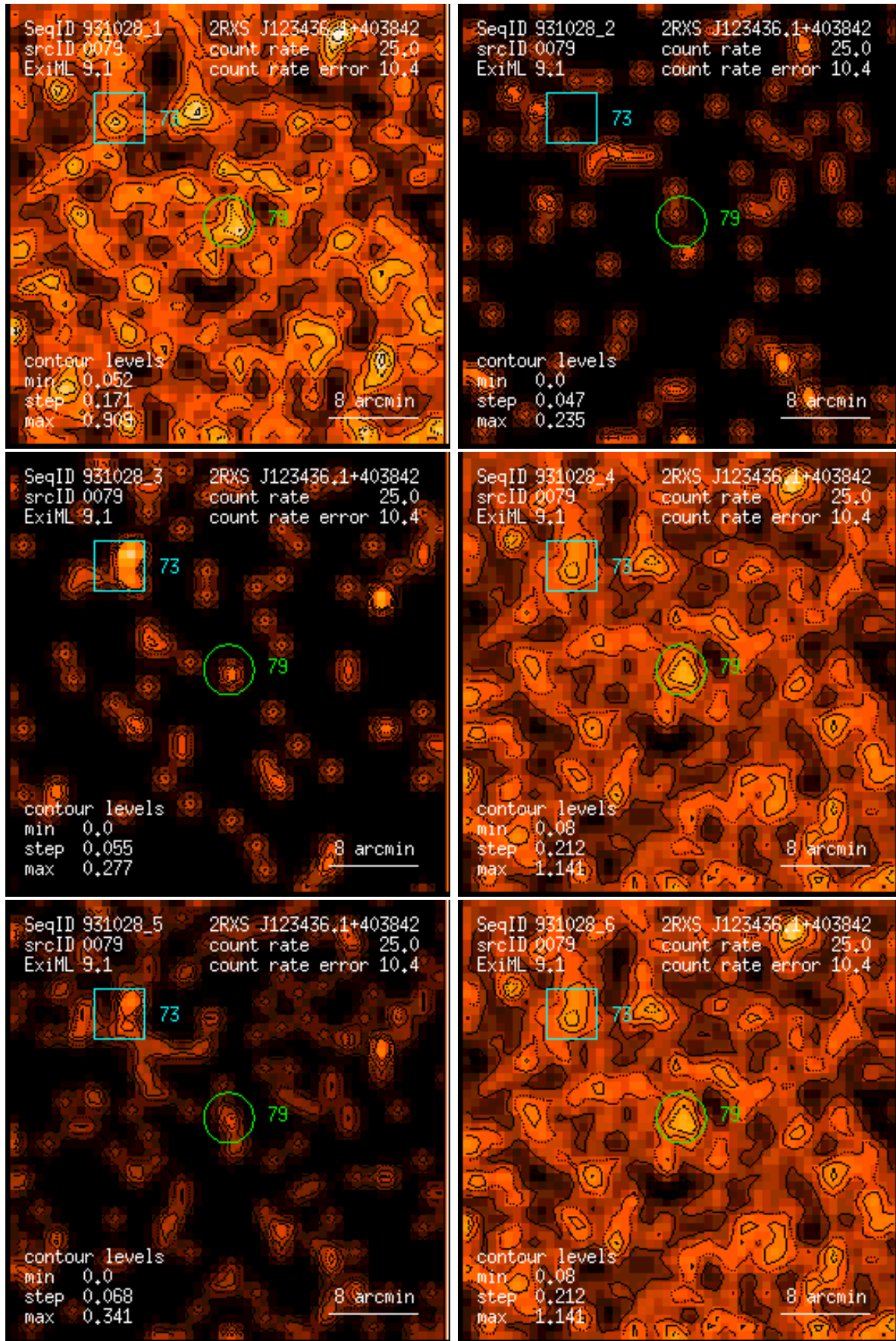
Figure 79: RASS 931028: detection 0079: band rate images, Gaussian filter: (1) PSPC channels 11 – 41, (2) 52 – 90, (3) 91 – 201, (4) 11 – 235, (5) 52 – 201, (6) 11 – 201. Broad band rates in counts/ks. Band rate contour levels in counts/ks/arcmin 2 .
