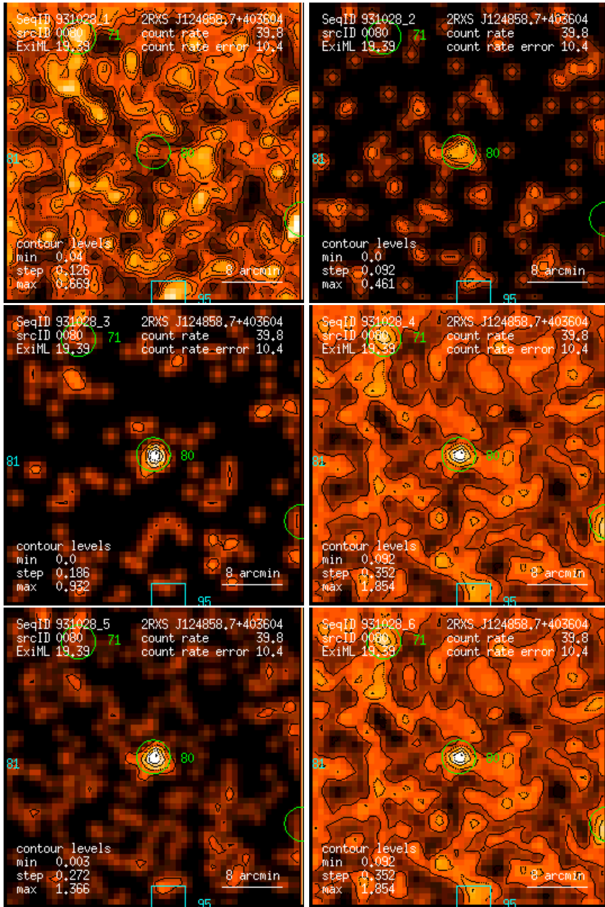
Figure 80: RASS 931028: detection 0080: band rate images, Gaussian filter: (1) PSPC channels 11 – 41, (2) 52 – 90, (3) 91 – 201, (4) 11 – 235, (5) 52 – 201, (6) 11 – 201. Broad band rates in counts/ks. Band rate contour levels in counts/ks/arcmin 2 .
