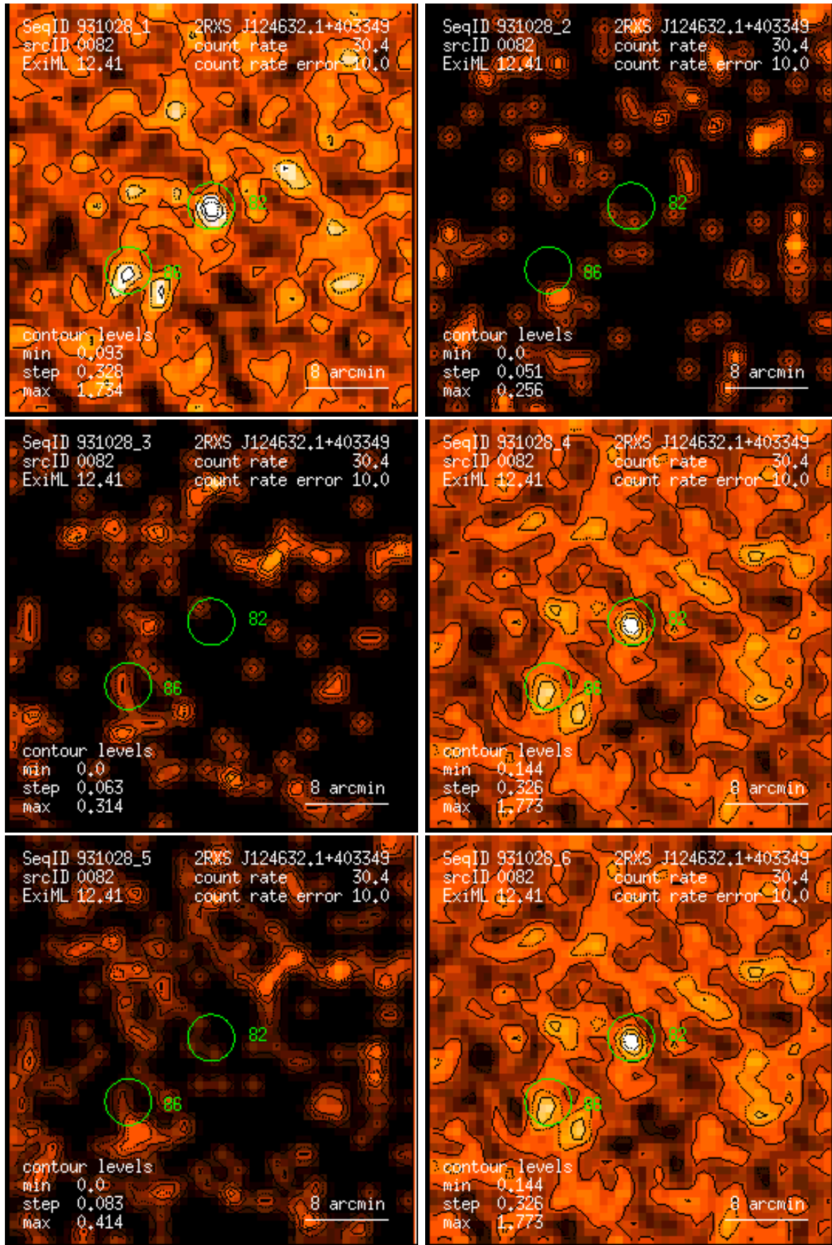
Figure 82: RASS 931028: detection 0082: band rate images, Gaussian filter: (1) PSPC channels 11 – 41, (2) 52 – 90, (3) 91 – 201, (4) 11 – 235, (5) 52 – 201, (6) 11 – 201. Broad band rates in counts/ks. Band rate contour levels in counts/ks/arcmin 2 .
