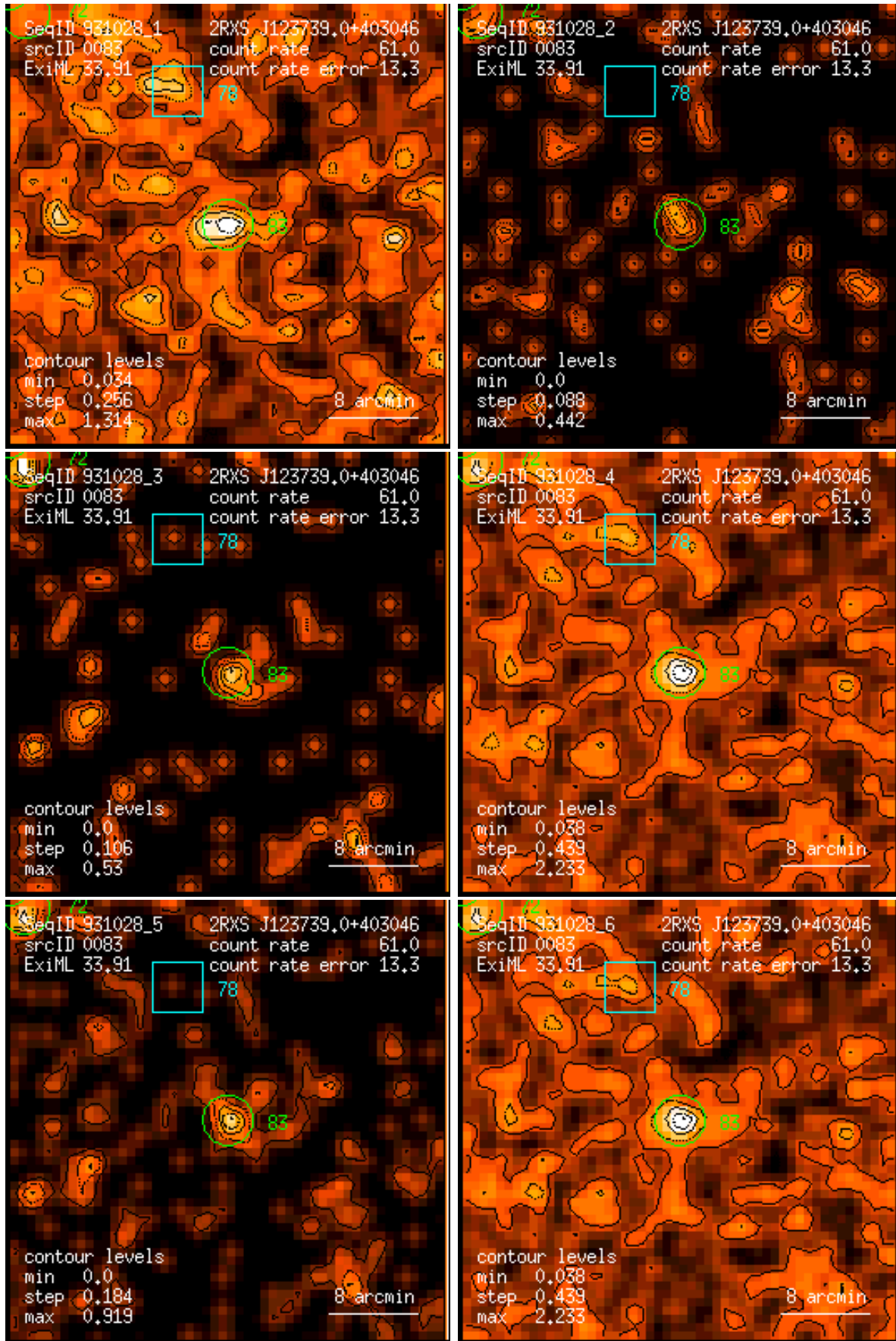
Figure 83: RASS 931028: detection 0083: band rate images, Gaussian filter: (1) PSPC channels 11 – 41, (2) 52 – 90, (3) 91 – 201, (4) 11 – 235, (5) 52 – 201, (6) 11 – 201. Broad band rates in counts/ks. Band rate contour levels in counts/ks/arcmin 2 .
