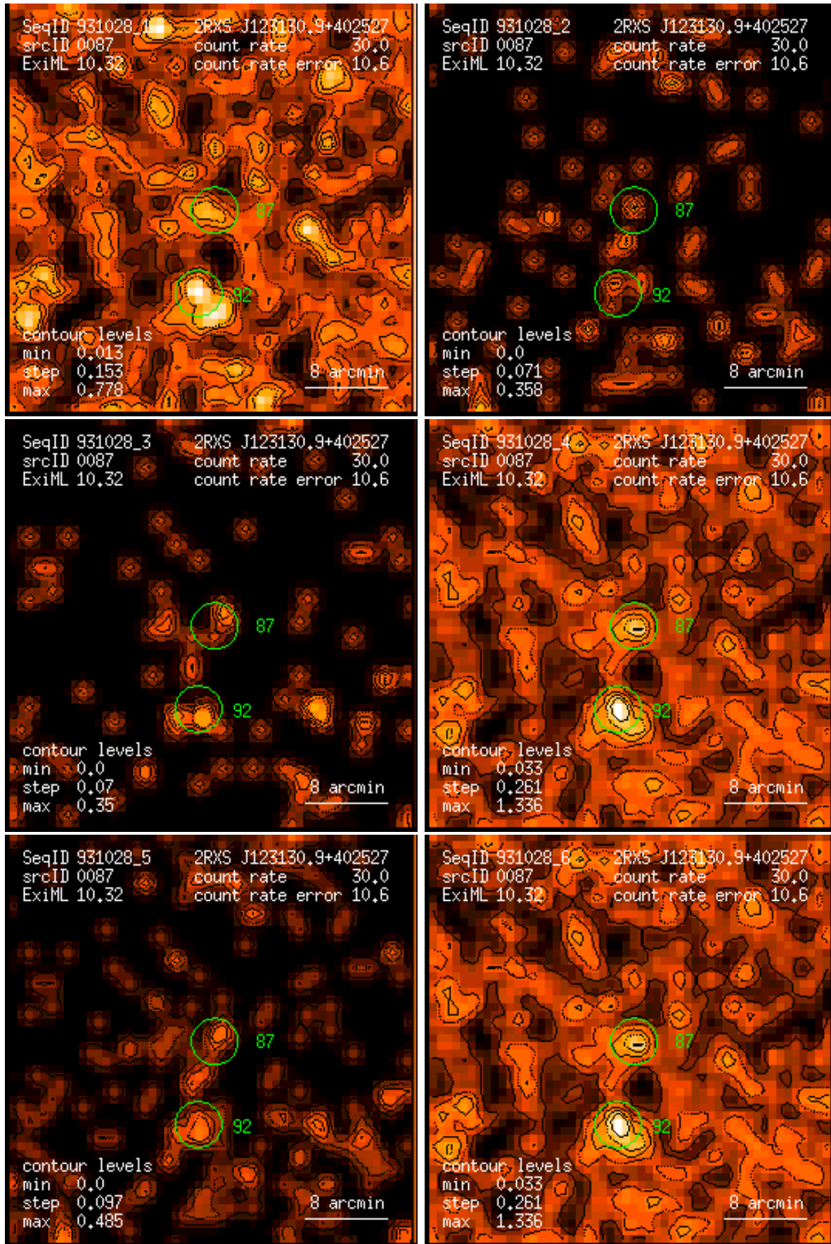
Figure 87: RASS 931028: detection 0087: band rate images, Gaussian filter: (1) PSPC channels 11 – 41, (2) 52 – 90, (3) 91 – 201, (4) 11 – 235, (5) 52 – 201, (6) 11 – 201. Broad band rates in counts/ks. Band rate contour levels in counts/ks/arcmin 2 .
