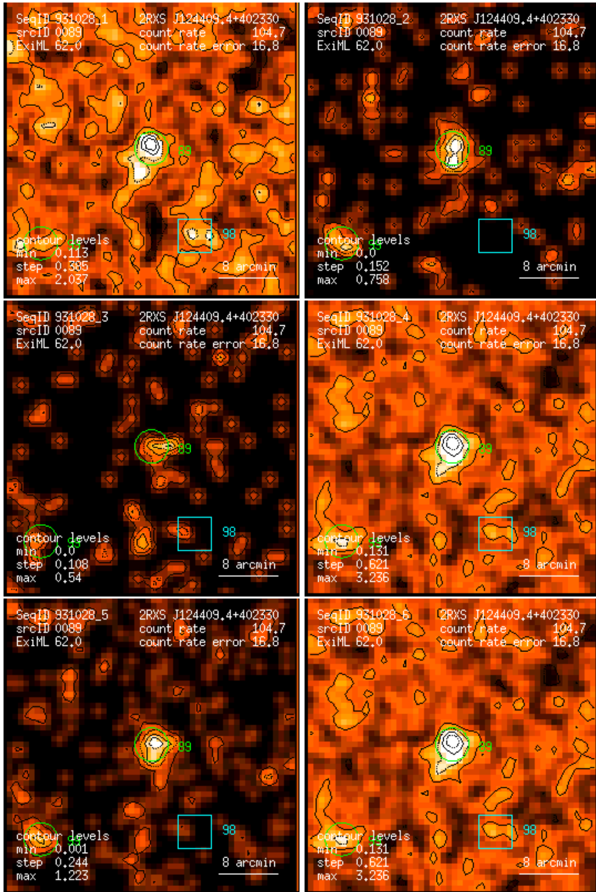
Figure 89: RASS 931028: detection 0089: band rate images, Gaussian filter: (1) PSPC channels 11 – 41, (2) 52 – 90, (3) 91 – 201, (4) 11 – 235, (5) 52 – 201, (6) 11 – 201. Broad band rates in counts/ks. Band rate contour levels in counts/ks/arcmin 2 .
