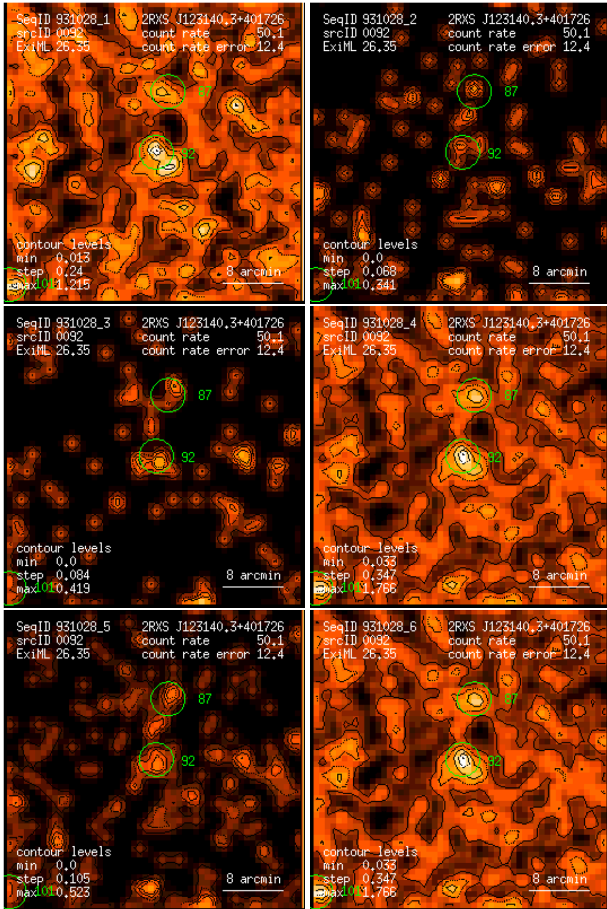
Figure 92: RASS 931028: detection 0092: band rate images, Gaussian filter: (1) PSPC channels 11 – 41, (2) 52 – 90, (3) 91 – 201, (4) 11 – 235, (5) 52 – 201, (6) 11 – 201. Broad band rates in counts/ks. Band rate contour levels in counts/ks/arcmin 2 .
