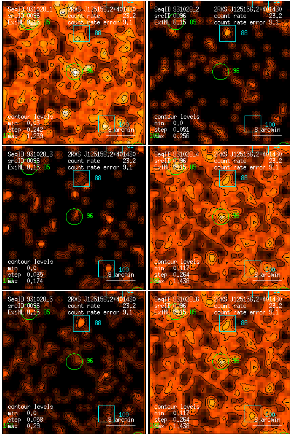
Figure 96: RASS 931028: detection 0096: band rate images, Gaussian filter: (1) PSPC channels 11 – 41, (2) 52 – 90, (3) 91 – 201, (4) 11 – 235, (5) 52 – 201, (6) 11 – 201. Broad band rates in counts/ks. Band rate contour levels in counts/ks/arcmin 2 .
