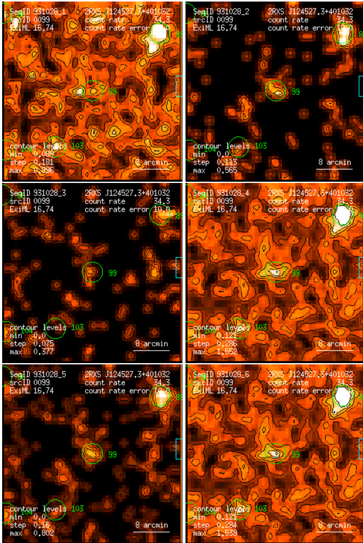
Figure 99: RASS 931028: detection 0099: band rate images, Gaussian filter: (1) PSPC channels 11 – 41, (2) 52 – 90, (3) 91 – 201, (4) 11 – 235, (5) 52 – 201, (6) 11 – 201. Broad band rates in counts/ks. Band rate contour levels in counts/ks/arcmin 2 .
