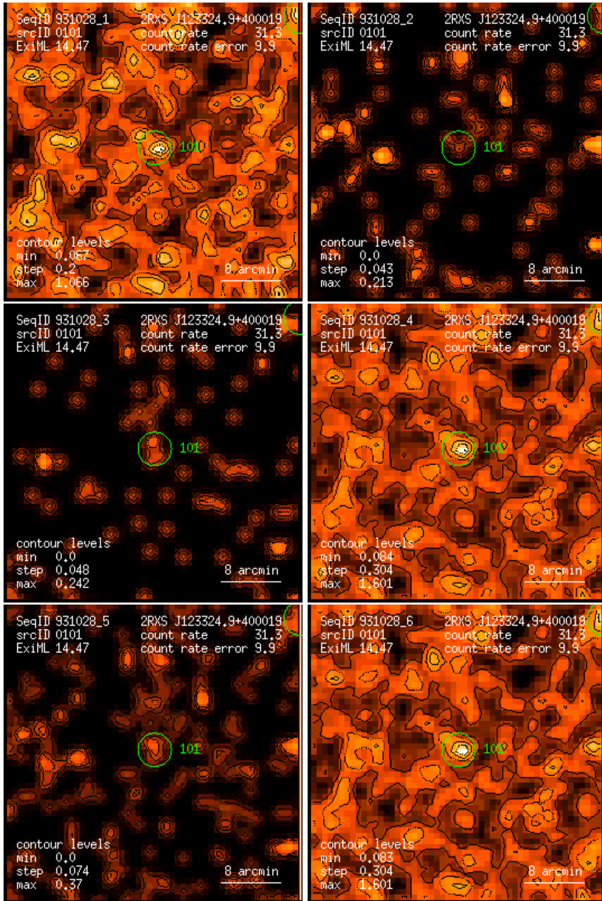
Figure 101: RASS 931028: detection 0101: band rate images, Gaussian filter: (1) PSPC channels 11 – 41, (2) 52 – 90, (3) 91 – 201, (4) 11 – 235, (5) 52 – 201, (6) 11 – 201. Broad band rates in counts/ks. Band rate contour levels in counts/ks/arcmin 2 .
