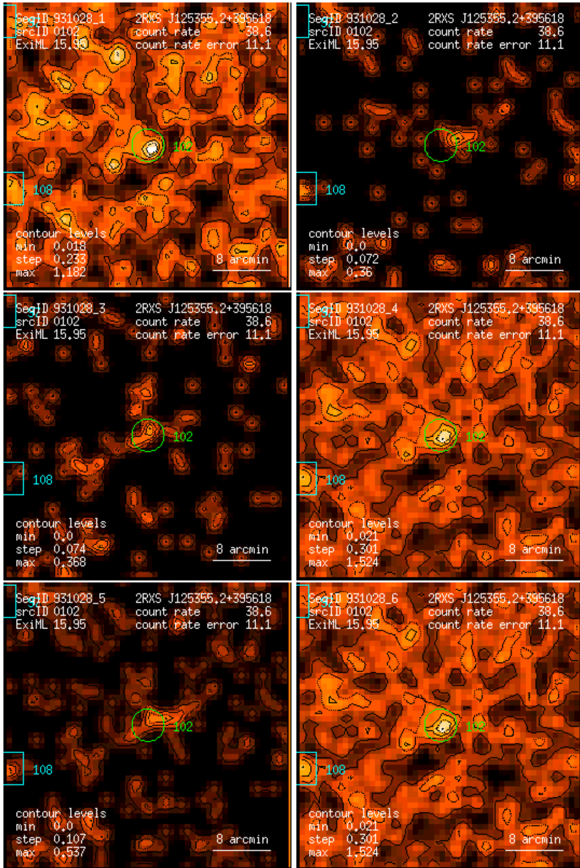
Figure 102: RASS 931028: detection 0102: band rate images, Gaussian filter: (1) PSPC channels 11 – 41, (2) 52 – 90, (3) 91 – 201, (4) 11 – 235, (5) 52 – 201, (6) 11 – 201. Broad band rates in counts/ks. Band rate contour levels in counts/ks/arcmin 2 .
