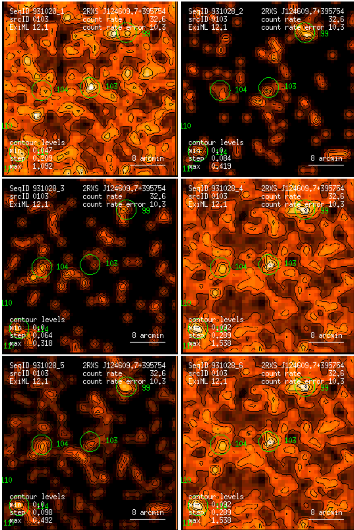
Figure 103: RASS 931028: detection 0103: band rate images, Gaussian filter: (1) PSPC channels 11 – 41, (2) 52 – 90, (3) 91 – 201, (4) 11 – 235, (5) 52 – 201, (6) 11 – 201. Broad band rates in counts/ks. Band rate contour levels in counts/ks/arcmin 2 .
