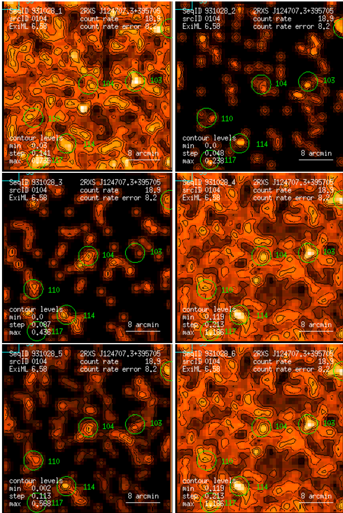
Figure 104: RASS 931028: detection 0104: band rate images, Gaussian filter: (1) PSPC channels 11 – 41, (2) 52 – 90, (3) 91 – 201, (4) 11 – 235, (5) 52 – 201, (6) 11 – 201. Broad band rates in counts/ks. Band rate contour levels in counts/ks/arcmin 2 .
