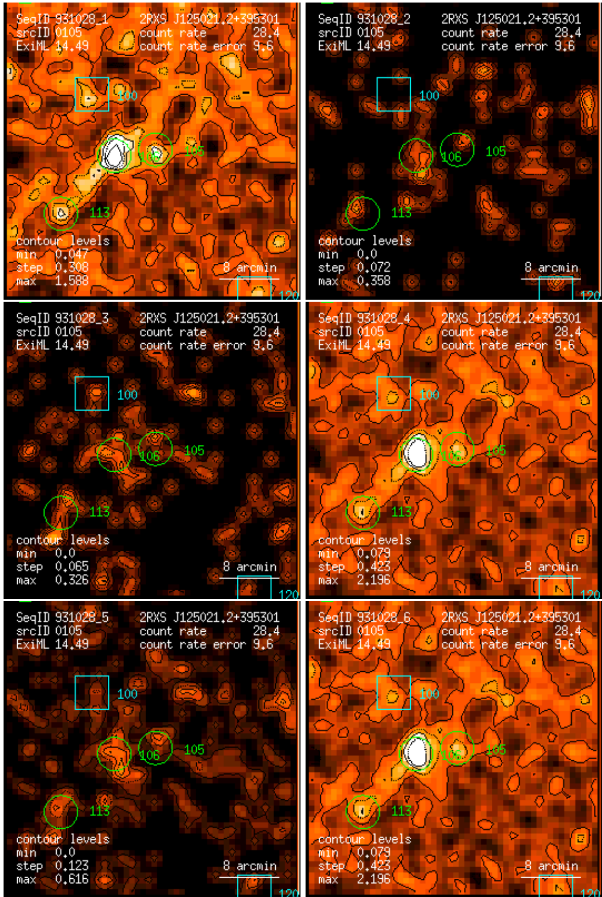
Figure 105: RASS 931028: detection 0105: band rate images, Gaussian filter: (1) PSPC channels 11 – 41, (2) 52 – 90, (3) 91 – 201, (4) 11 – 235, (5) 52 – 201, (6) 11 – 201. Broad band rates in counts/ks. Band rate contour levels in counts/ks/arcmin 2 .
