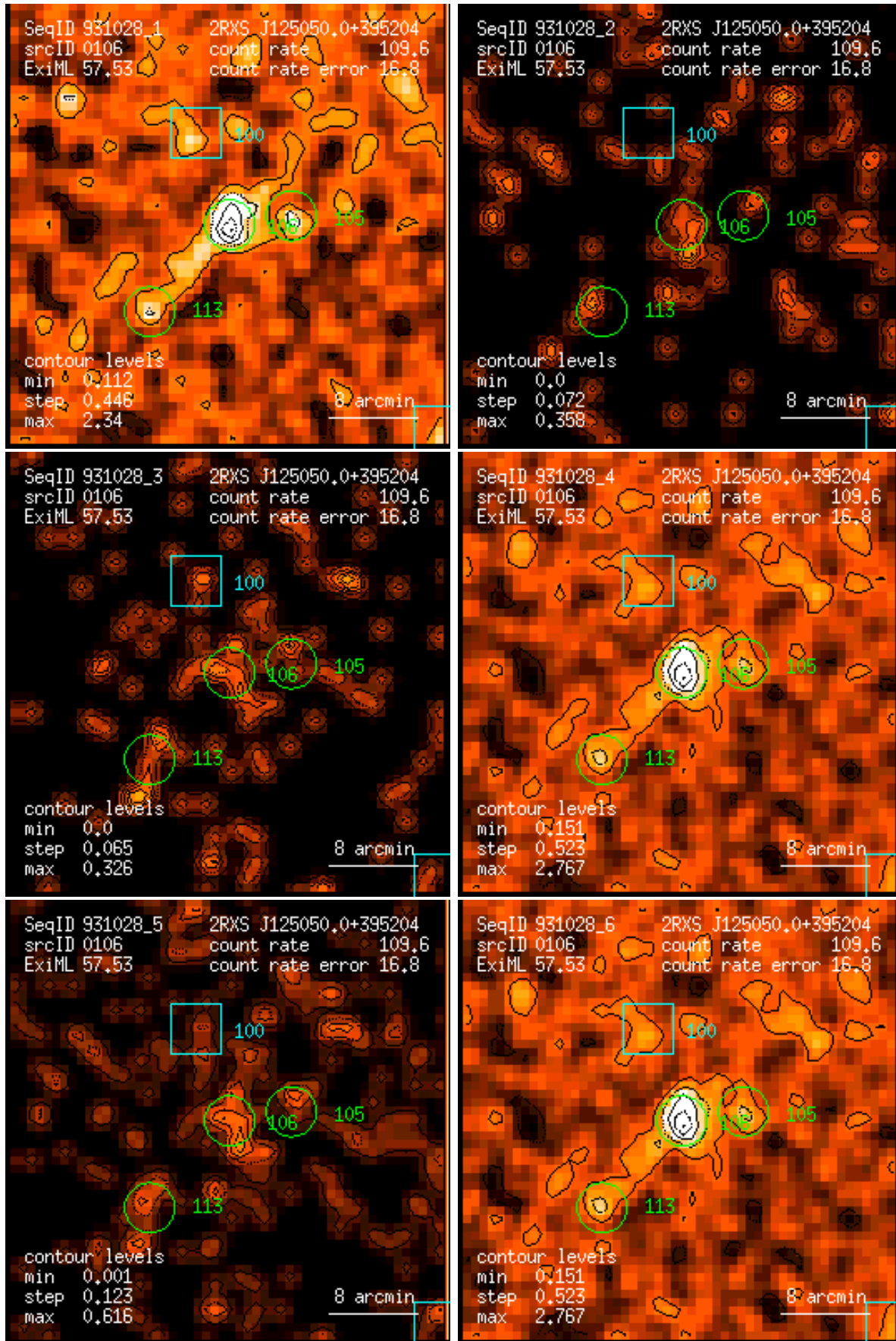
Figure 106: RASS 931028: detection 0106: band rate images, Gaussian filter: (1) PSPC channels 11 – 41, (2) 52 – 90, (3) 91 – 201, (4) 11 – 235, (5) 52 – 201, (6) 11 – 201. Broad band rates in counts/ks. Band rate contour levels in counts/ks/arcmin 2 .
