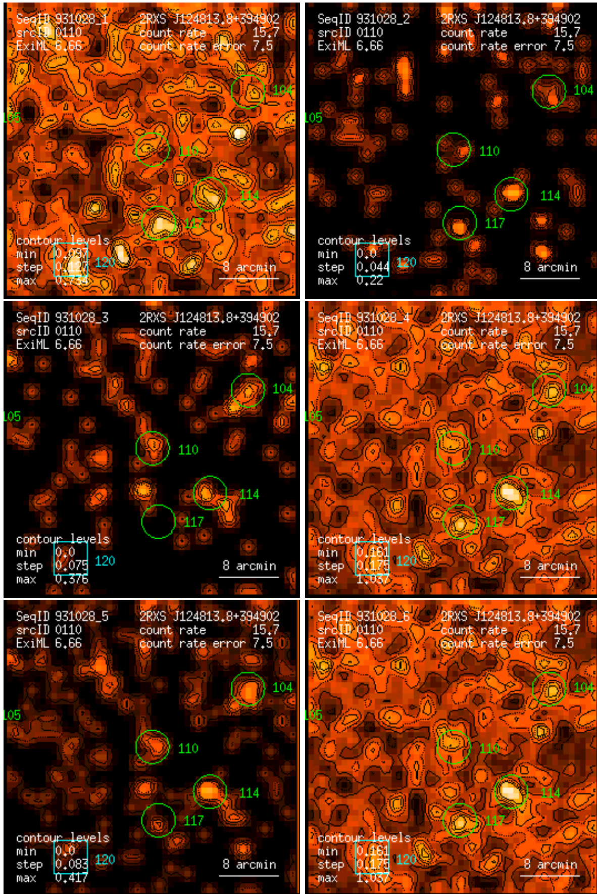
Figure 110: RASS 931028: detection 0110: band rate images, Gaussian filter: (1) PSPC channels 11 – 41, (2) 52 – 90, (3) 91 – 201, (4) 11 – 235, (5) 52 – 201, (6) 11 – 201. Broad band rates in counts/ks. Band rate contour levels in counts/ks/arcmin 2 .
