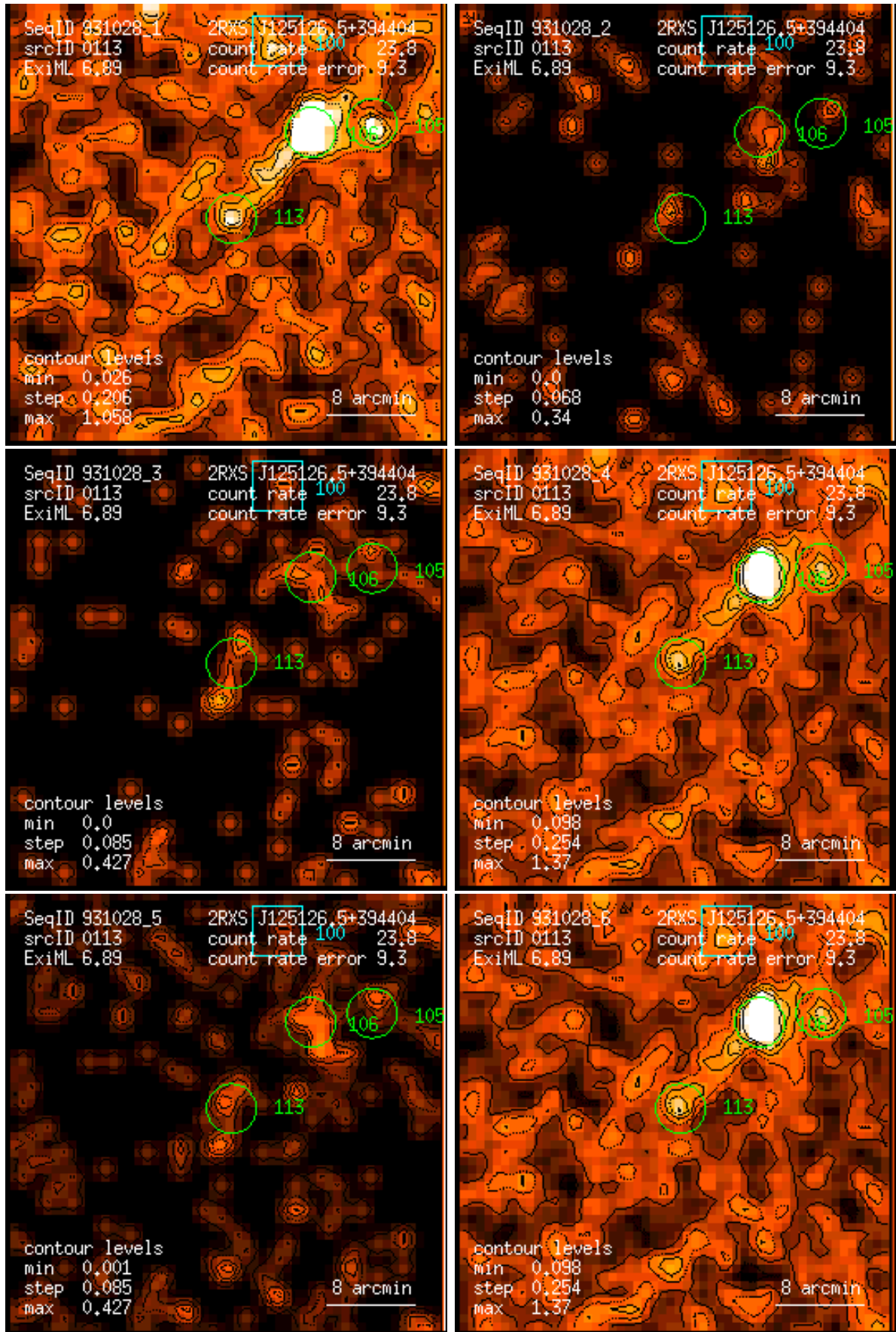
Figure 113: RASS 931028: detection 0113: band rate images, Gaussian filter: (1) PSPC channels 11 – 41, (2) 52 – 90, (3) 91 – 201, (4) 11 – 235, (5) 52 – 201, (6) 11 – 201. Broad band rates in counts/ks. Band rate contour levels in counts/ks/arcmin 2 .
